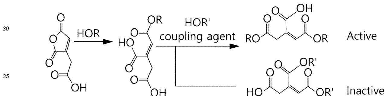
[Reaction scheme 2]
