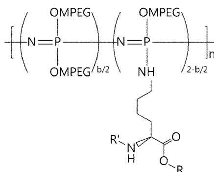
[Chemical formula 19]
