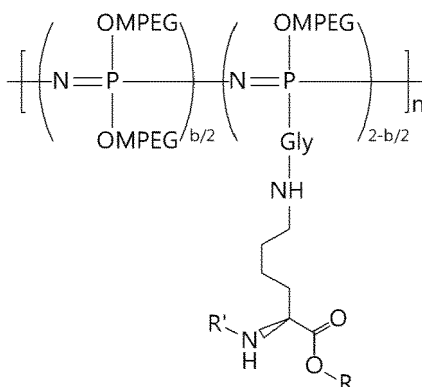
[Chemical formula 20]
