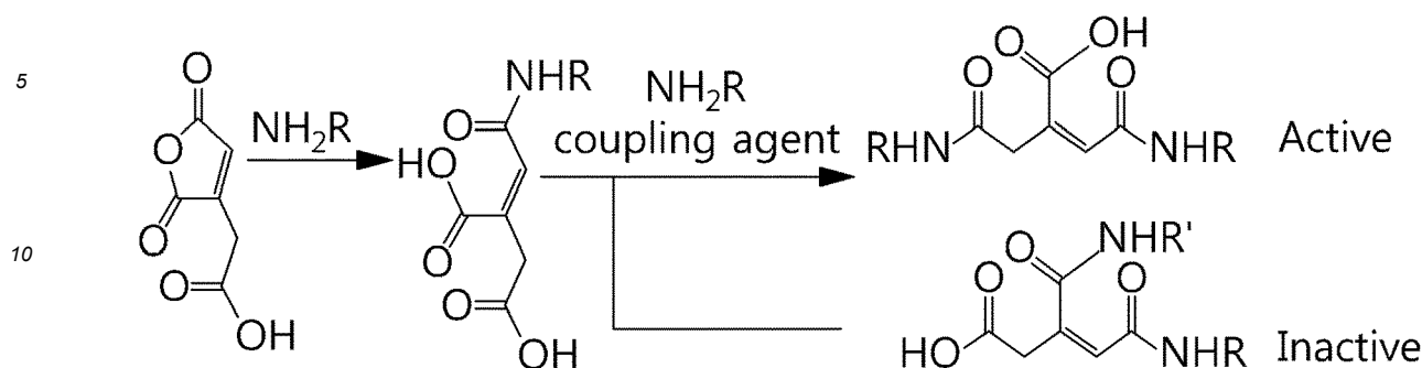
[Reaction scheme 1]
