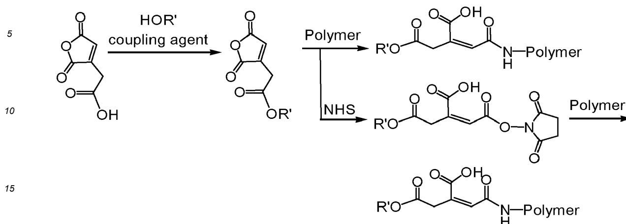
[Reaction scheme 3]
