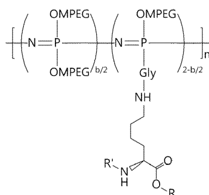
[Chemical formula 20]
