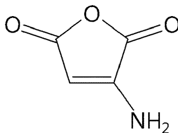
[Chemical formula 8]
