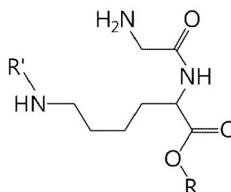
[Chemical formula 18]
