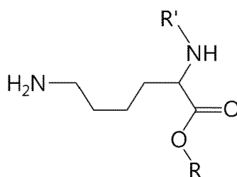
[Chemical formula 17]
