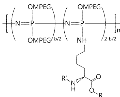
[Chemical formula 20]
