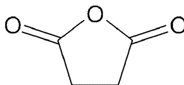
[Chemical formula 11]
