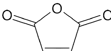
[Chemical formula 10]
