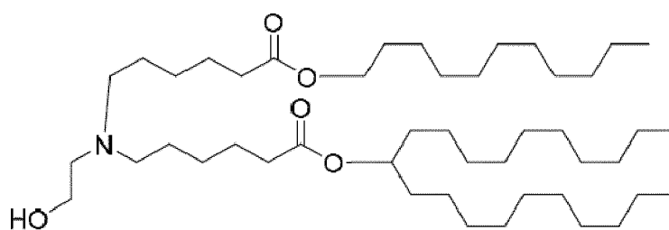
(Compound 185),
