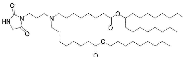
(Compound 174),
