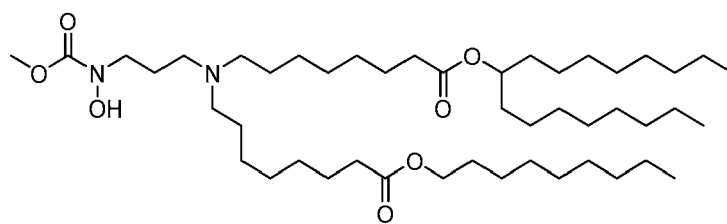
(Compound 205),
