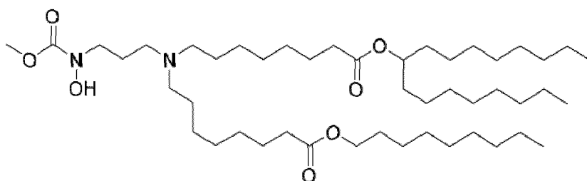
(Compound 205),
