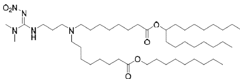
(Compound 209),
