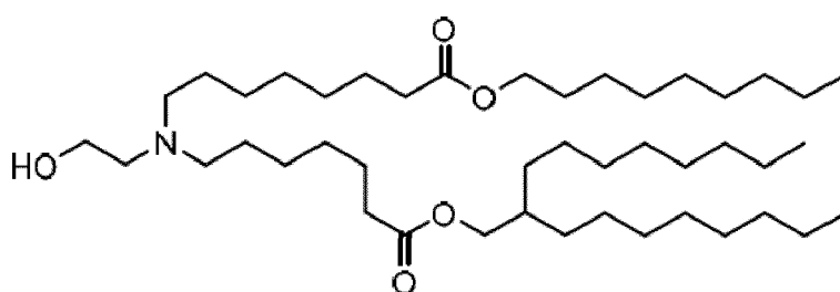
(Compound 143),
