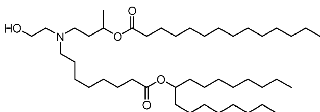
(Compound 99),
