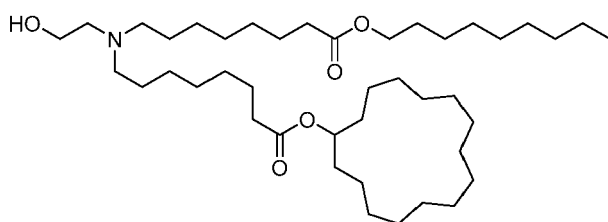
(Compound 81),
