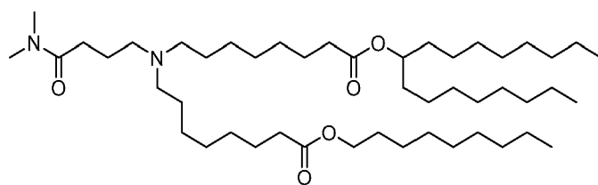
(Compound 224),
