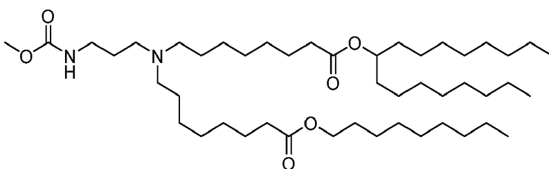
(Compound 181),
