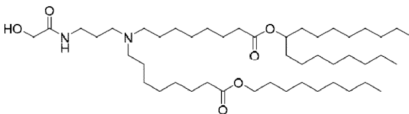
(Compound 198),
