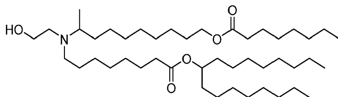
(Compound 161),
