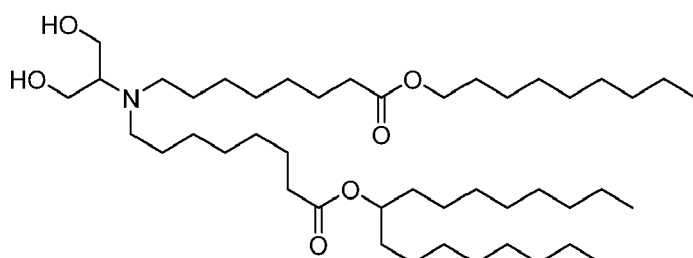
(Compound 156),
