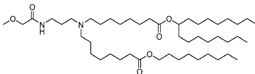
(Compound 178),
