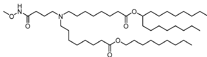
(Compound 226),
