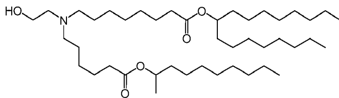
(Compound 122),
