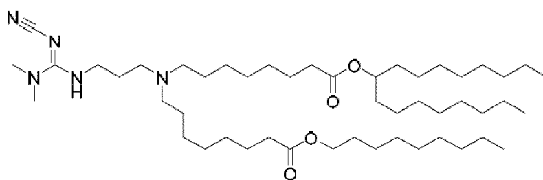
(Compound 168),
