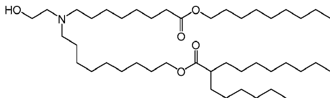
(Compound 134),
