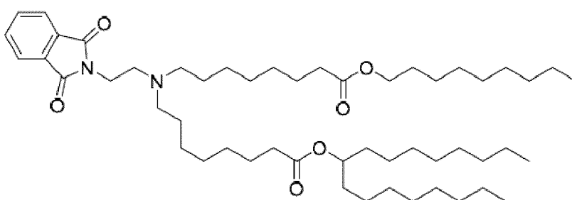
(Compound 100),
