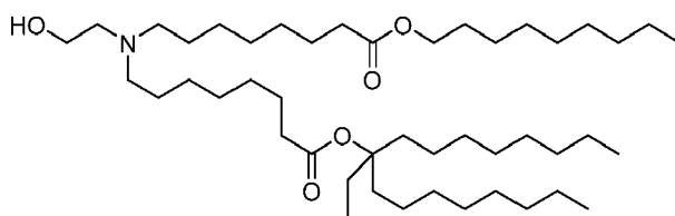
(Compound 83),
