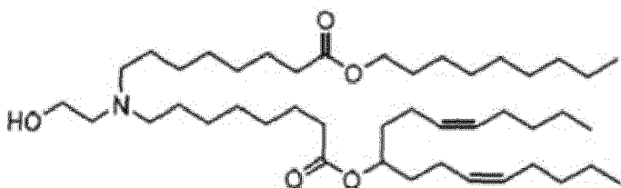
(Compound 60),
