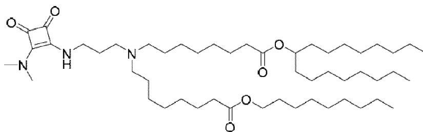
(Compound 169),
