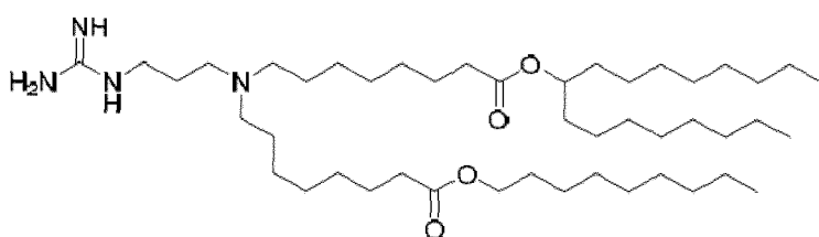
(Compound 207),
