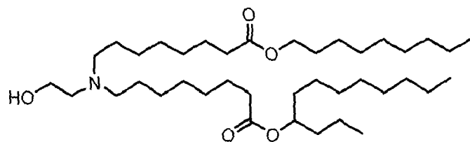
(Compound 34),
