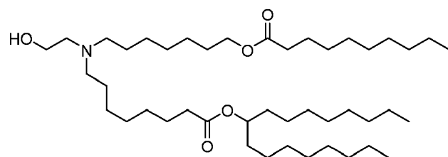
(Compound 96),
