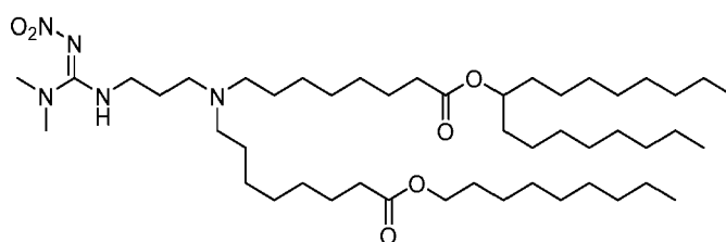
(Compound 209),
