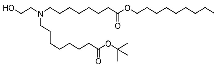
(Compound 158),
