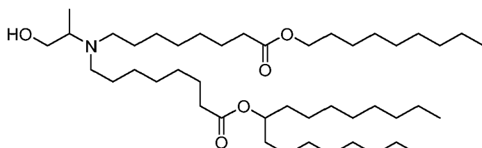
(Compound 157),
