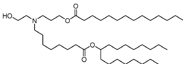
(Compound 97),
