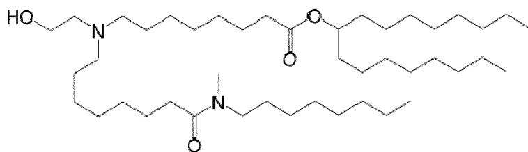
(Compound 145),
