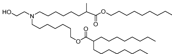
(Compound 163),
