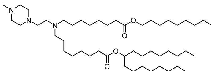
(Compound 101),
