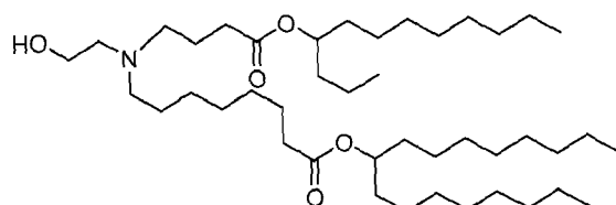
(Compound 74),
