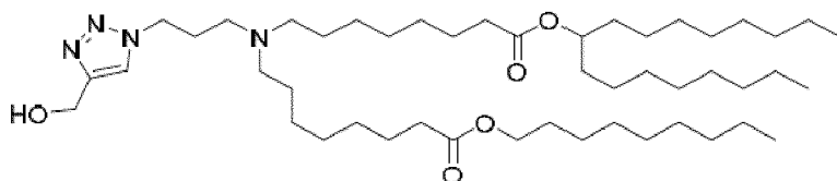
(Compound 218),
