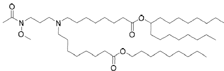
(Compound 203),
