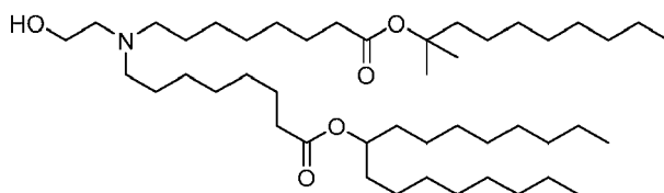
(Compound 85),
