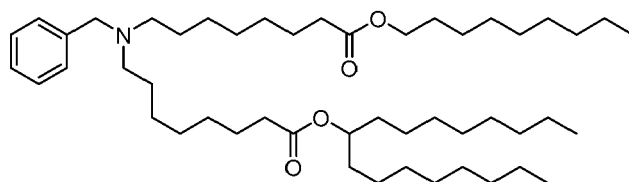
(Compound 94),
