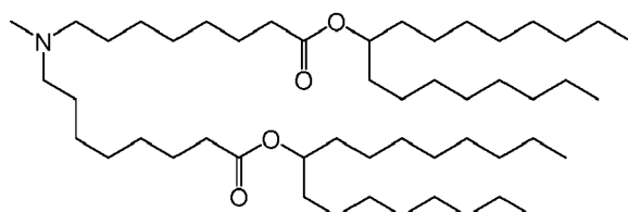
(Compound 124),
