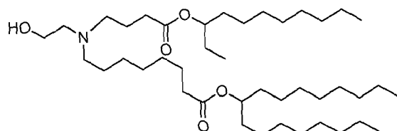
(Compound 72),
