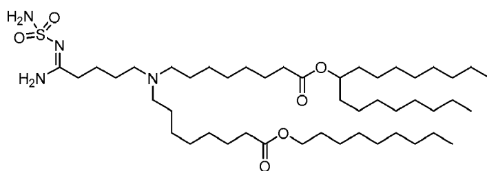
(Compound 221),
