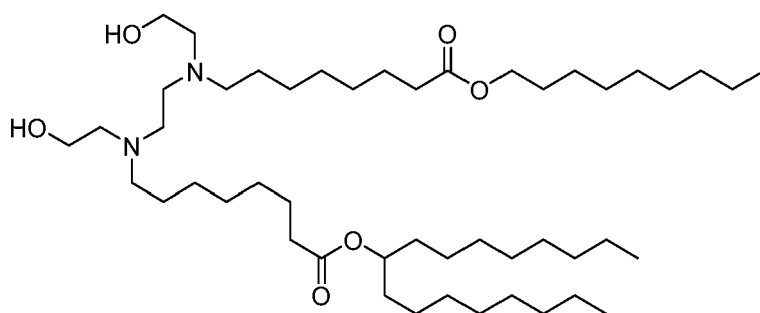
(Compound 159),
