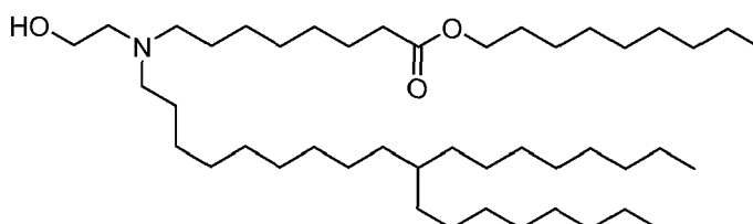
(Compound 153),
