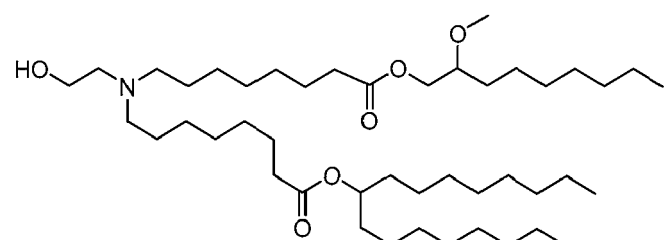
(Compound 148),
