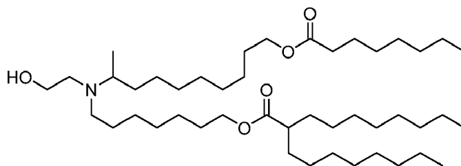
(Compound 162),
