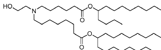
(Compound 77),
