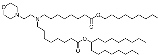
(Compound 103),
