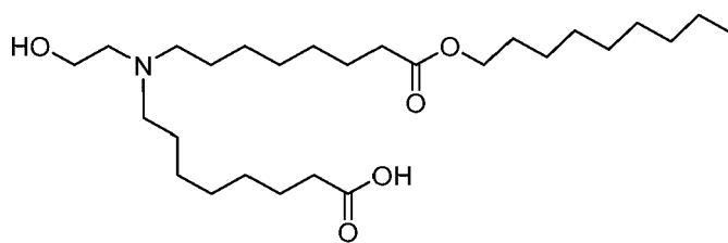
(Compound 167),
