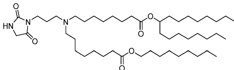
(Compound 174),
