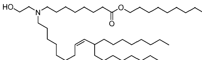
(Compound 152),
