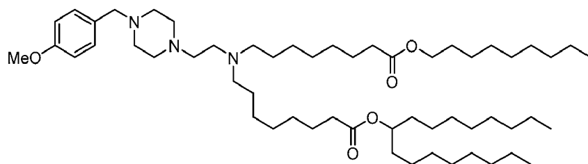
(Compound 102),
