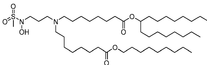
(Compound 206),
