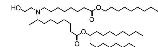
(Compound 217),
