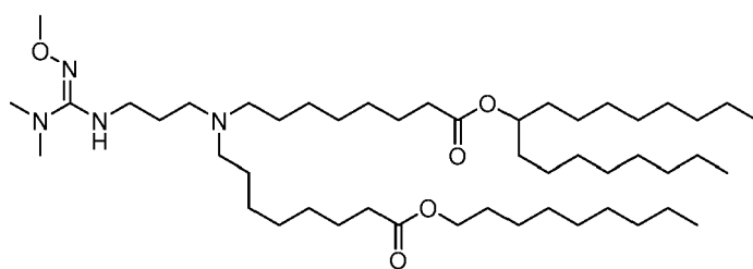
(Compound 211),
