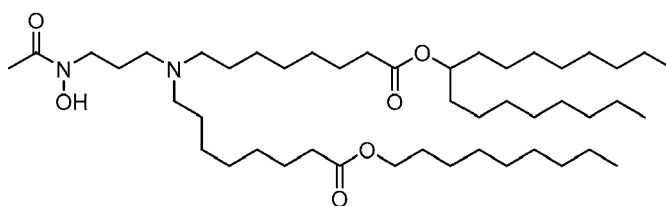
(Compound 204),
