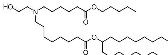
(Compound 104),
