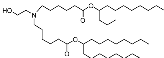
(Compound 92),
