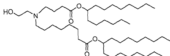
(Compound 73),
