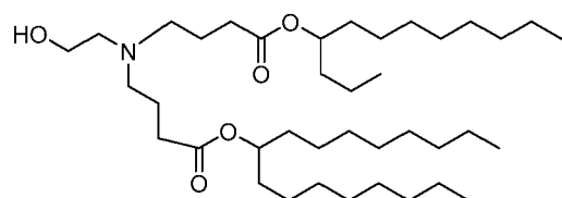
(Compound 90),
