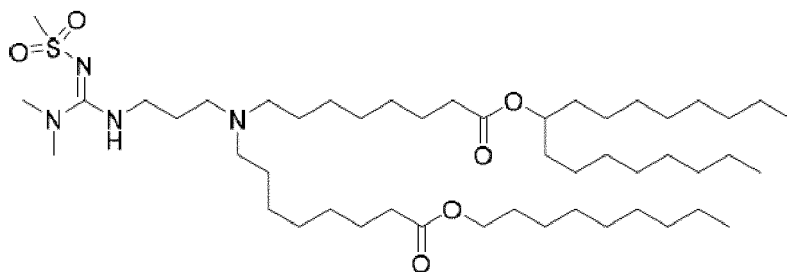
(Compound 213),
