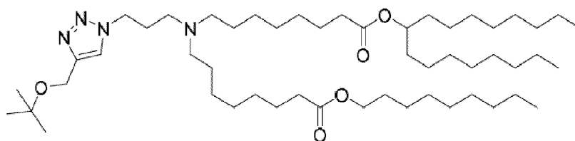
(Compound 177),
