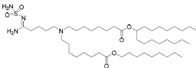
(Compound 221),
