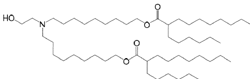
(Compound 133),
