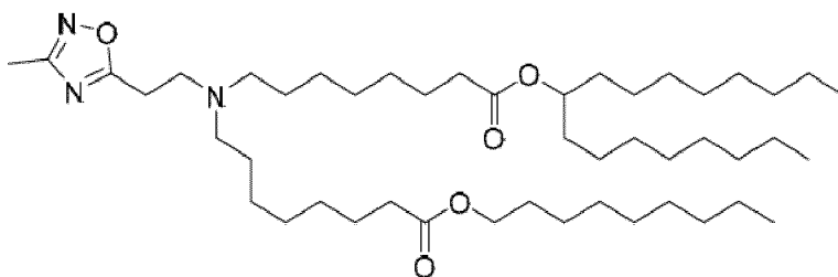
(Compound 230),
