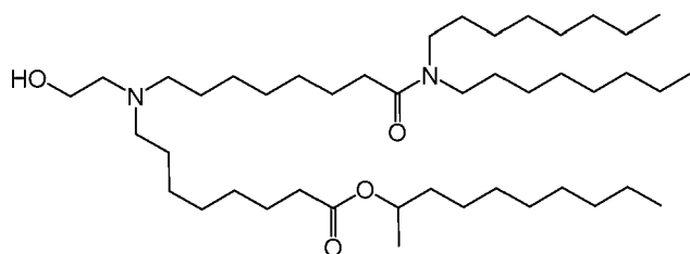
(Compound 130),
