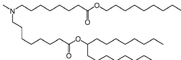
(Compound 123),
