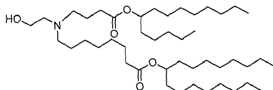
(Compound 71),
