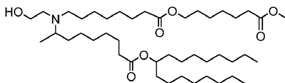
(Compound 192),
