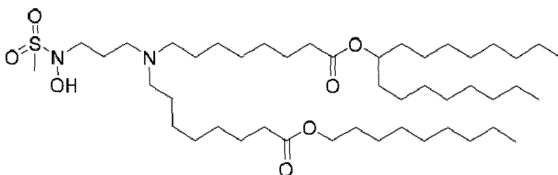
(Compound 206),
