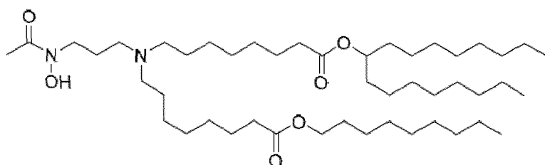
(Compound 204),
