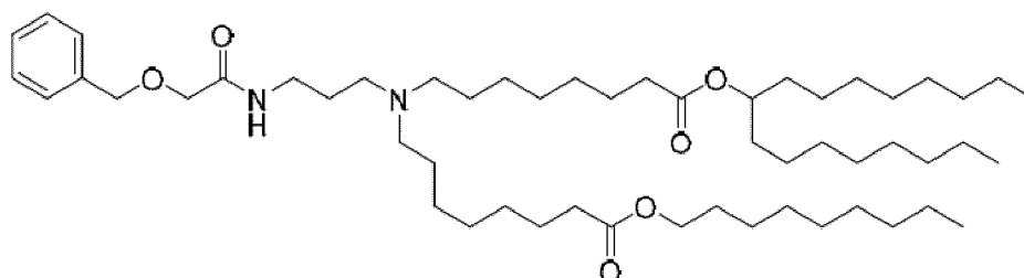
(Compound 197),
