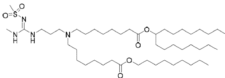
(Compound 212),
