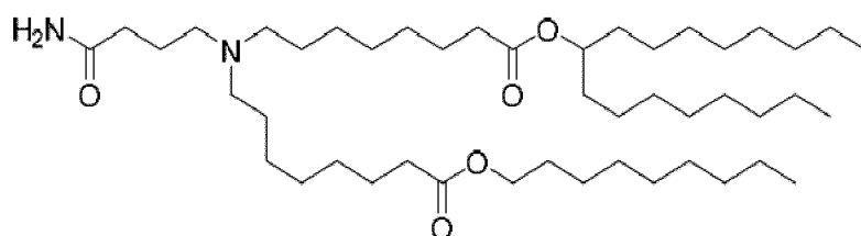
(Compound 222),
