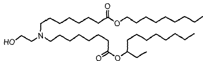
(Compound 35),
