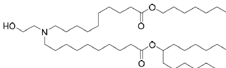
(Compound 186),
