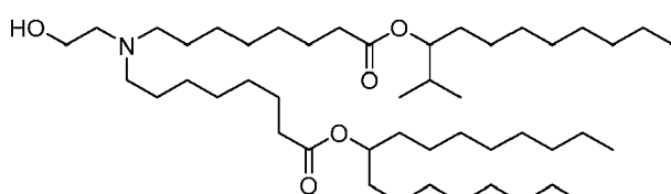
(Compound 78),
