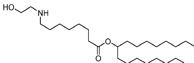
(Compound 180),
