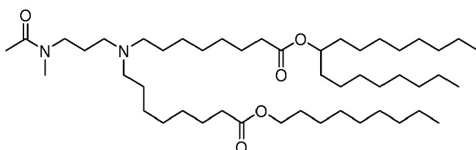
(Compound 196),
