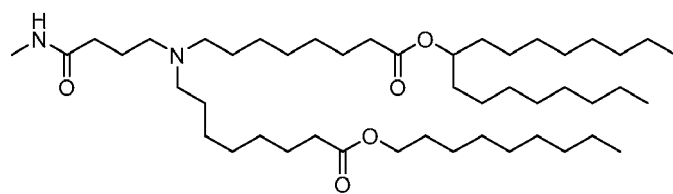
(Compound 223),
