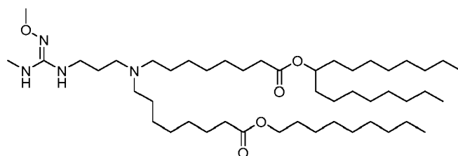
(Compound 210),
