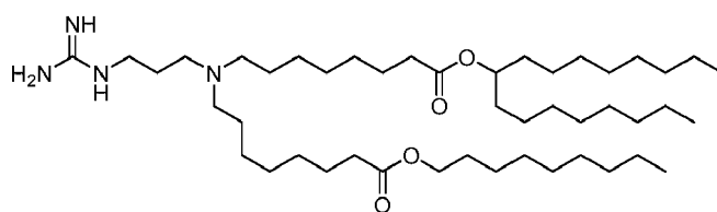
(Compound 207),
