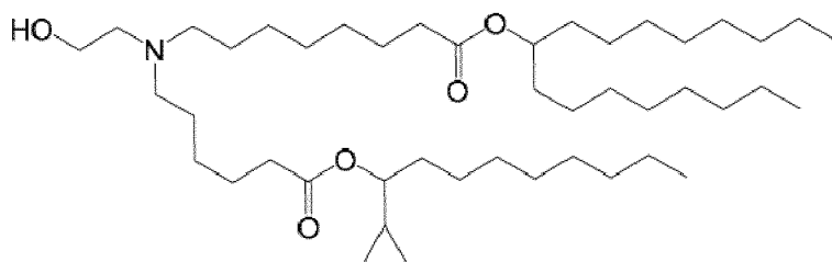
(Compound 128),
