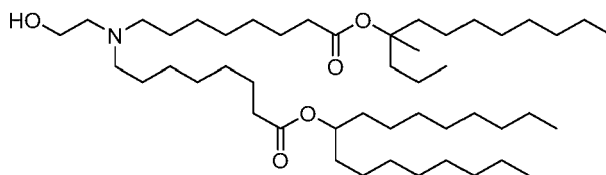
(Compound 87),
