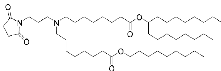
(Compound 176),
