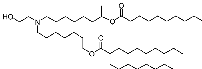
(Compound 165),
