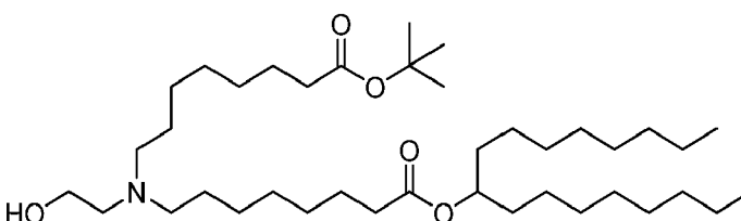
(Compound 155),
