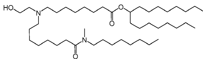
(Compound 145),
