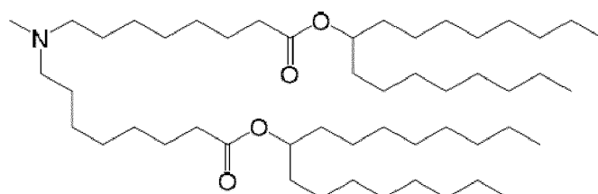
(Compound 124),
