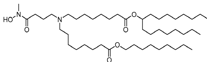
(Compound 227),
