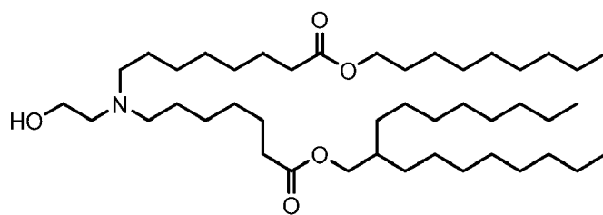
(Compound 143),
