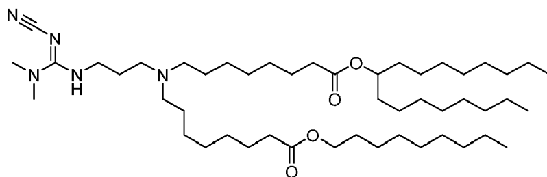
(Compound 168),
