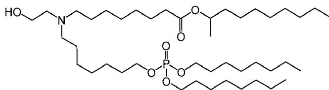
(Compound 132),
