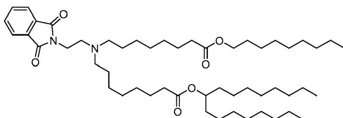
(Compound 100),
