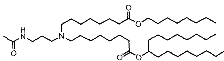
(Compound 37),
