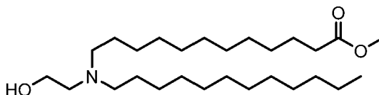
Methyl 12-(dodecyl(2-hydroxyethyl)amino)dodecanoate
