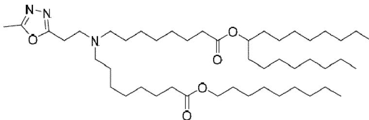
(Compound 231),
