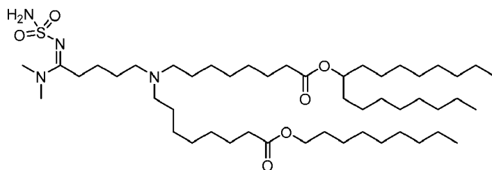
(Compound 219),
