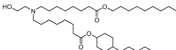
(Compound 79),
