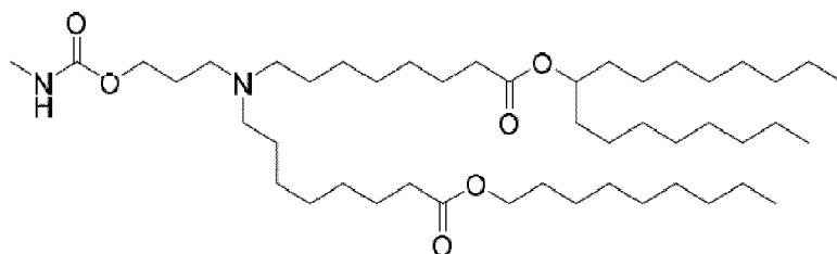
(Compound 175),
