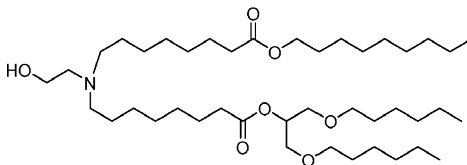
(Compound 183),
