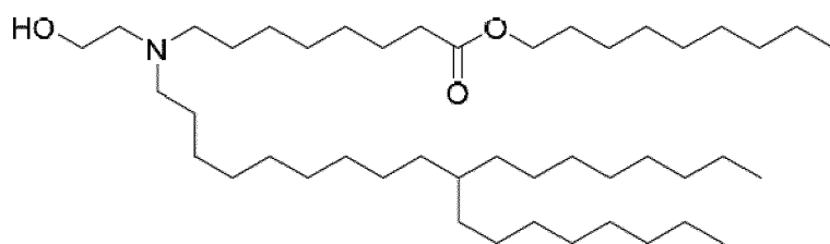
(Compound 153),
