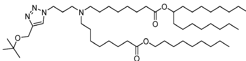
(Compound 177),
