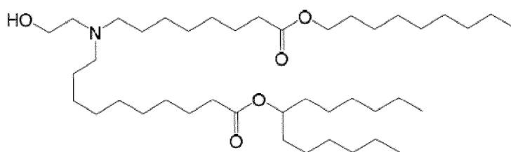
(Compound 147),
