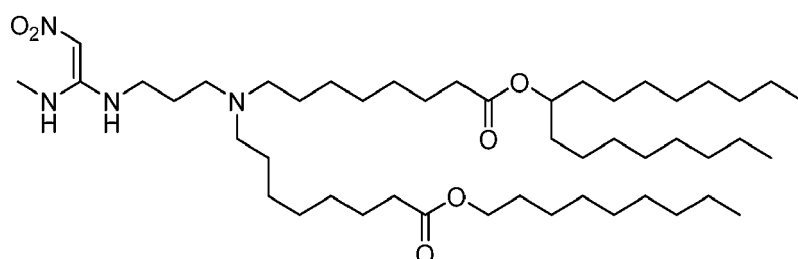
(Compound 170),
