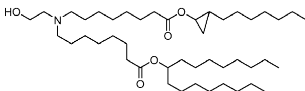
(Compound 93),
