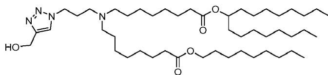
(Compound 218),
