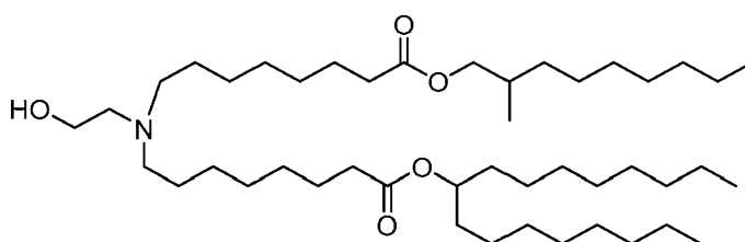
(Compound 184),
