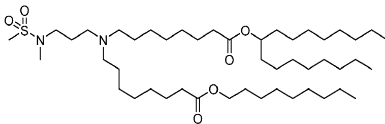
(Compound 173),
