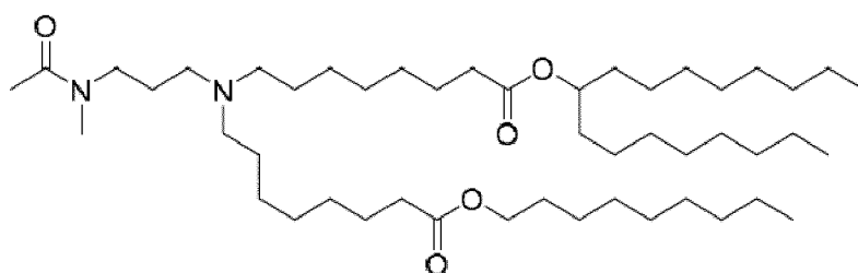
(Compound 196),
