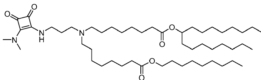
(Compound 169),
