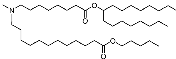
(Compound 150),
