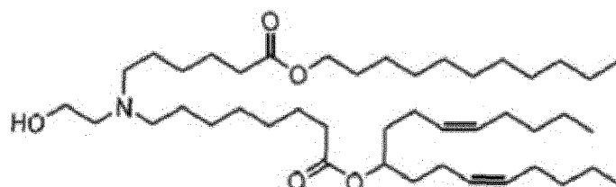
(Compound 61)
