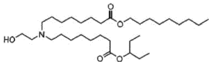
(Compound 59),
