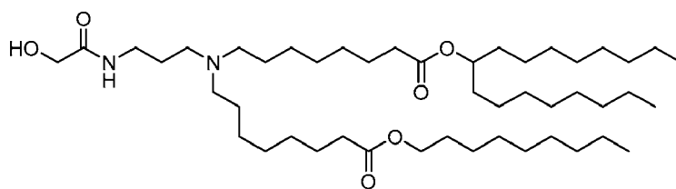
(Compound 198),
