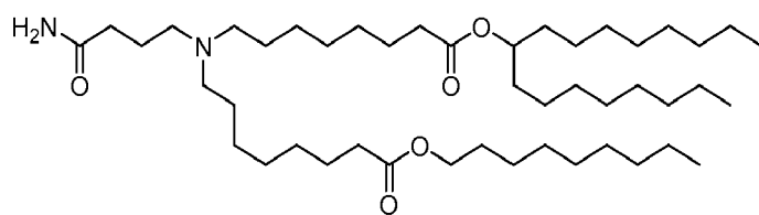
(Compound 222),
