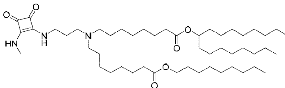
(Compound 182),
