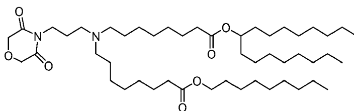
(Compound 202),
