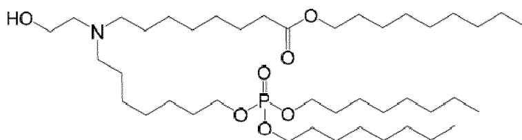
(Compound 131),
