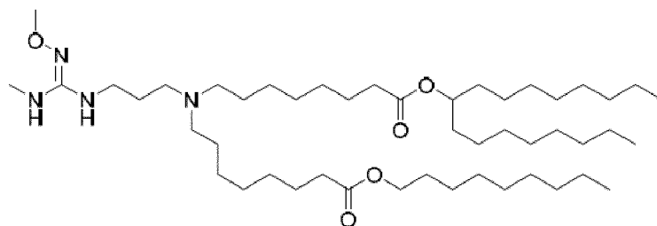
(Compound 210),
