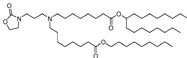
(Compound 199),
