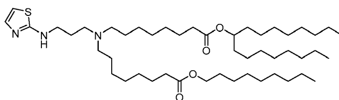
(Compound 208),
