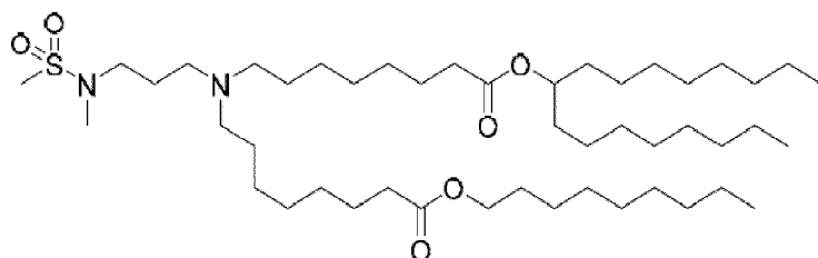
(Compound 173),
