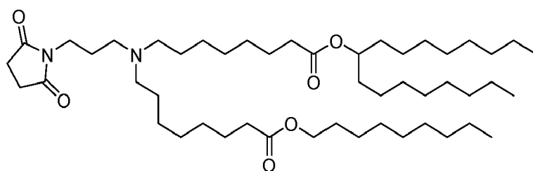
(Compound 176),
