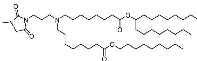
(Compound 201),
