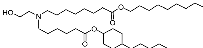
(Compound 232),
