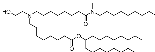
(Compound 105),
