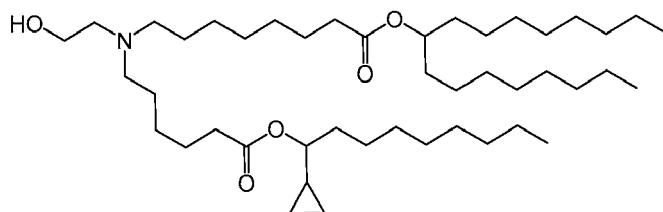
(Compound 128),
