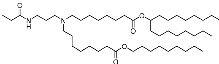
(Compound 193),
