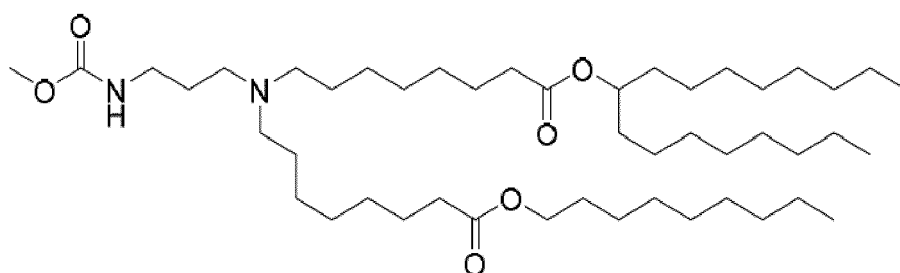
(Compound 181),
