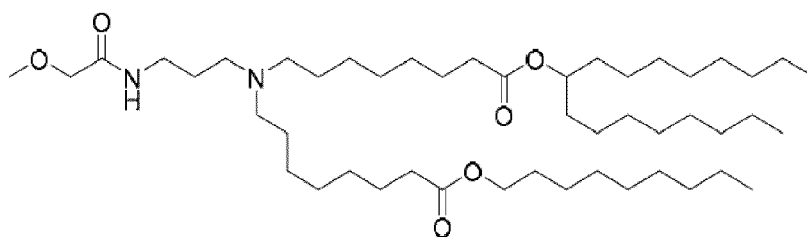
(Compound 178),
