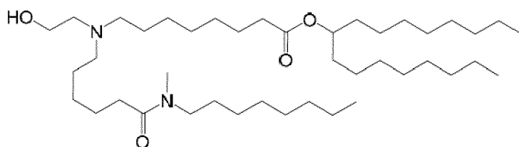
(Compound 146),
