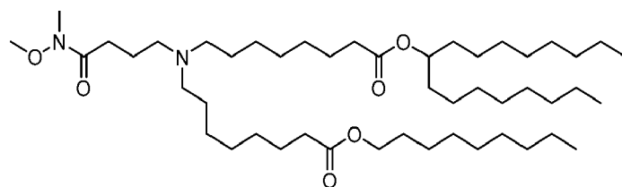
(Compound 228),
