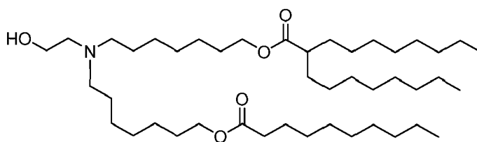
(Compound 151),
