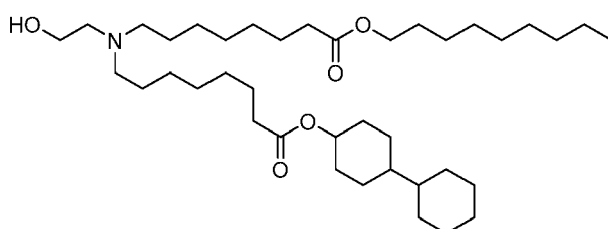
(Compound 80),
