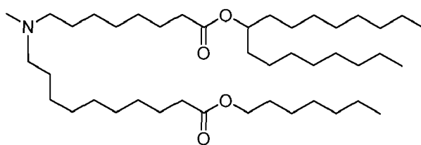
(Compound 149),
