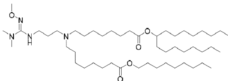
(Compound 211),
