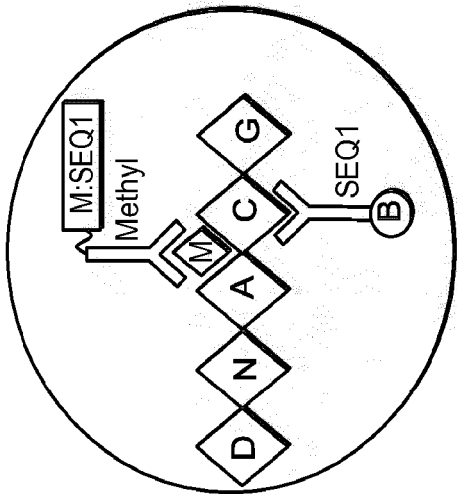
FIG. 37J Methyl or 3-OH Methyl:DNA
