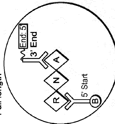
FIG. 37F RNA Full length
