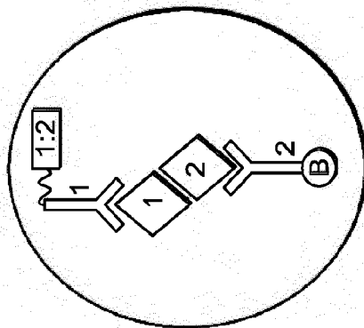
FIG. 37B Complex
