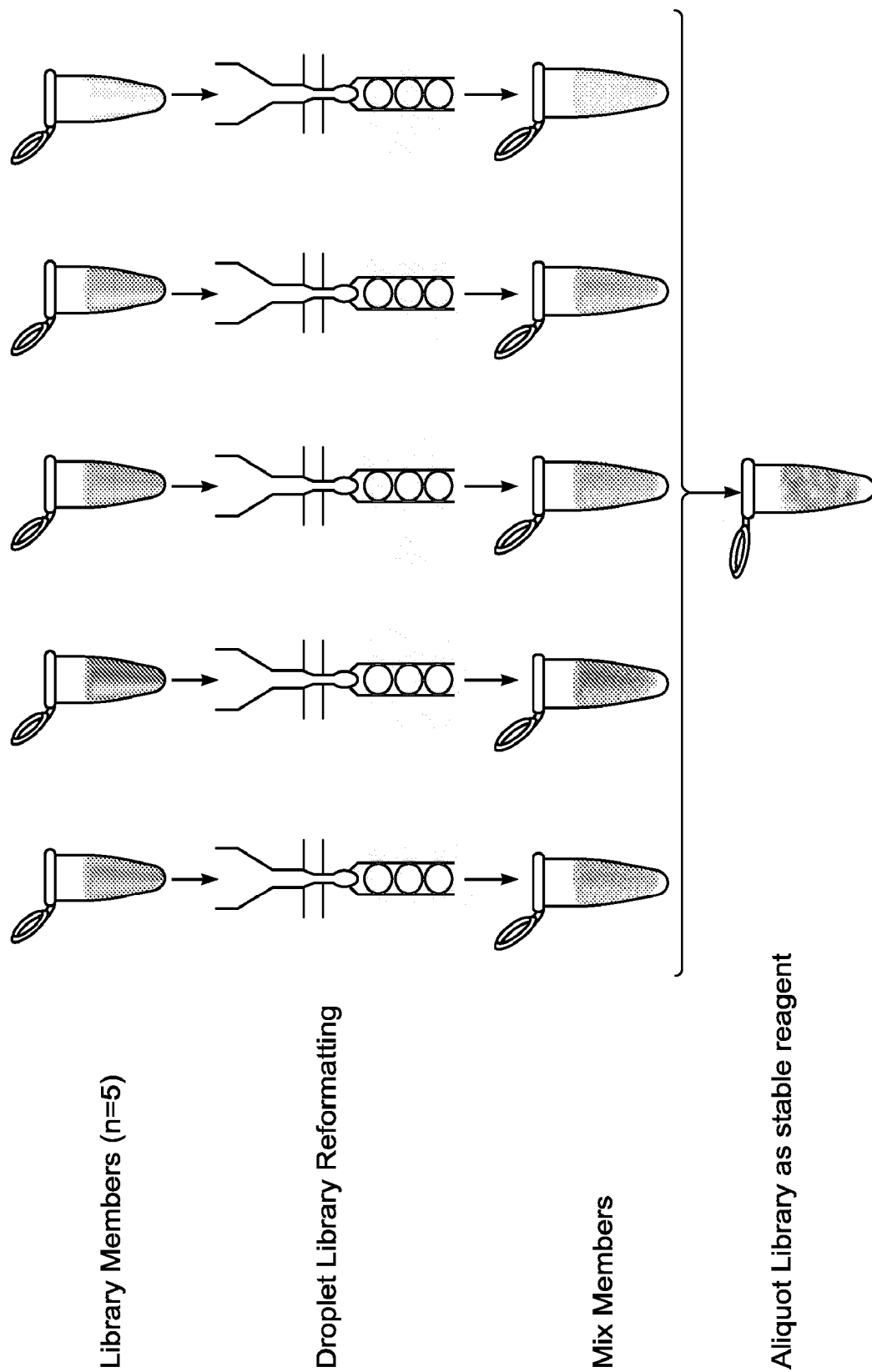
FIG. 72A Reagents: Oligos, DNA, Antibodies, Enzymes, Serum, Compounds, Virus, Cells
