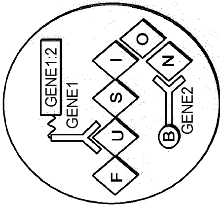
FIG. 37I DNA Gene fusion
