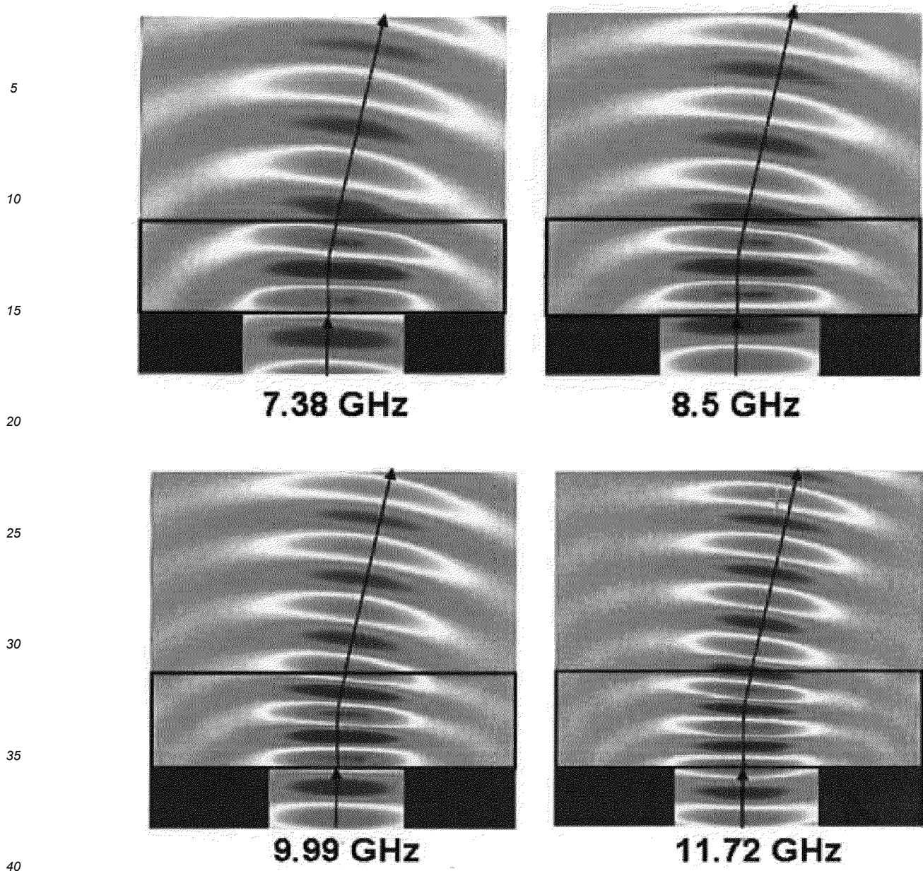
Fig. 5. Field mapping measurements of the beam steering lens. The lens has a linear gradient that causes the incoming beam to be deflected by an angle of 16.2 degrees. The effect is broadband, as can be seen from the identical maps taken at four different frequencies that span the X-band range of the experimental apparatus.
