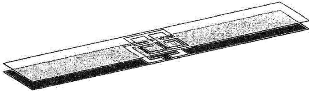
Figure 3: Wave-guided Complimentary Negative Index Metamaterials
