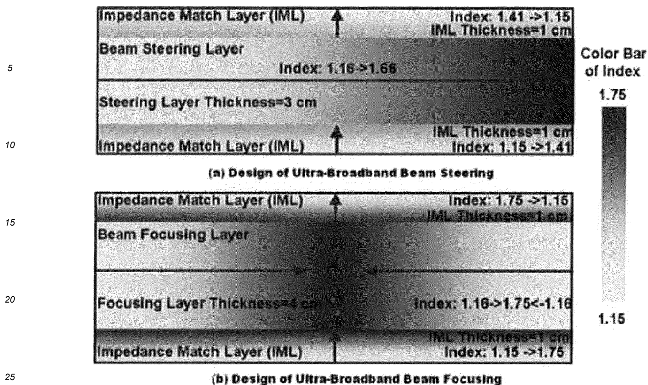
Fig. 3. Refractive index distributions for the designed gradient index structures. (a) A beam-steering element based on a linear index gradient. (b) A beam focusing lens, based on a higher order polynomial index gradient. Note the presence in both designs of an impedance matching layer (IML), provided to improve the insertion loss of the structures.
