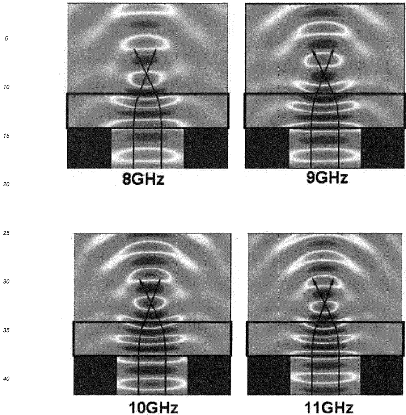
Fig. 6. Field mapping measurements of the beam focusing lens. The lens has a symmetric profile about the center (given in the text) that causes the incoming beam to be focused to a point. Once again, the function is broadband, as can be seen from the identical maps taken at four different frequencies that span the X-band range of the experimental apparatus.
