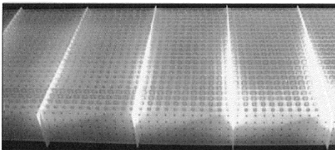
Fig. 4. Fabricated sample, in which, the metamaterial structures vary with space coordinate.
