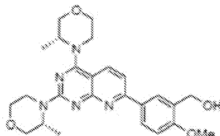
AZD8055
