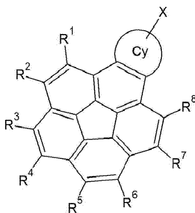
[Chemical Formula 1]
