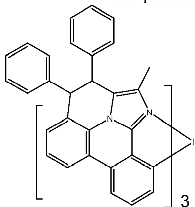
Compound 54
