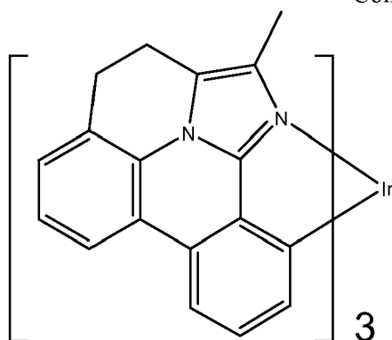
Compound 86
