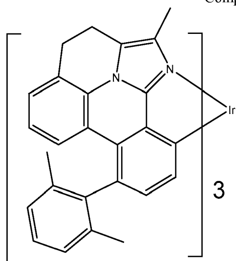
Compound 94
