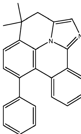
Compound (1-37)
