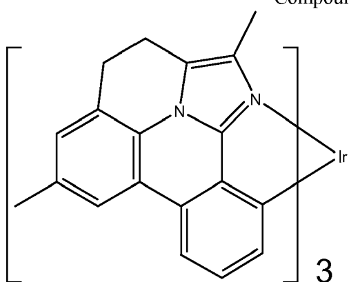
Compound 93
