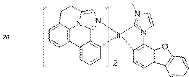
Compound 21
