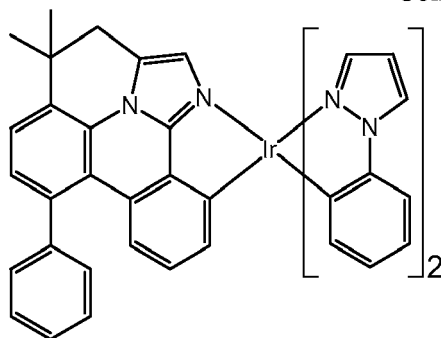
Compound 50
