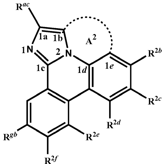
Formula (2b)
