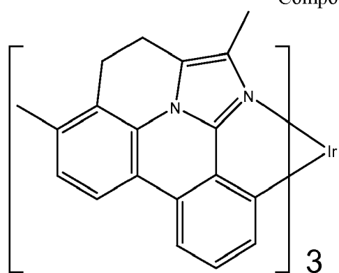
Compound 92
