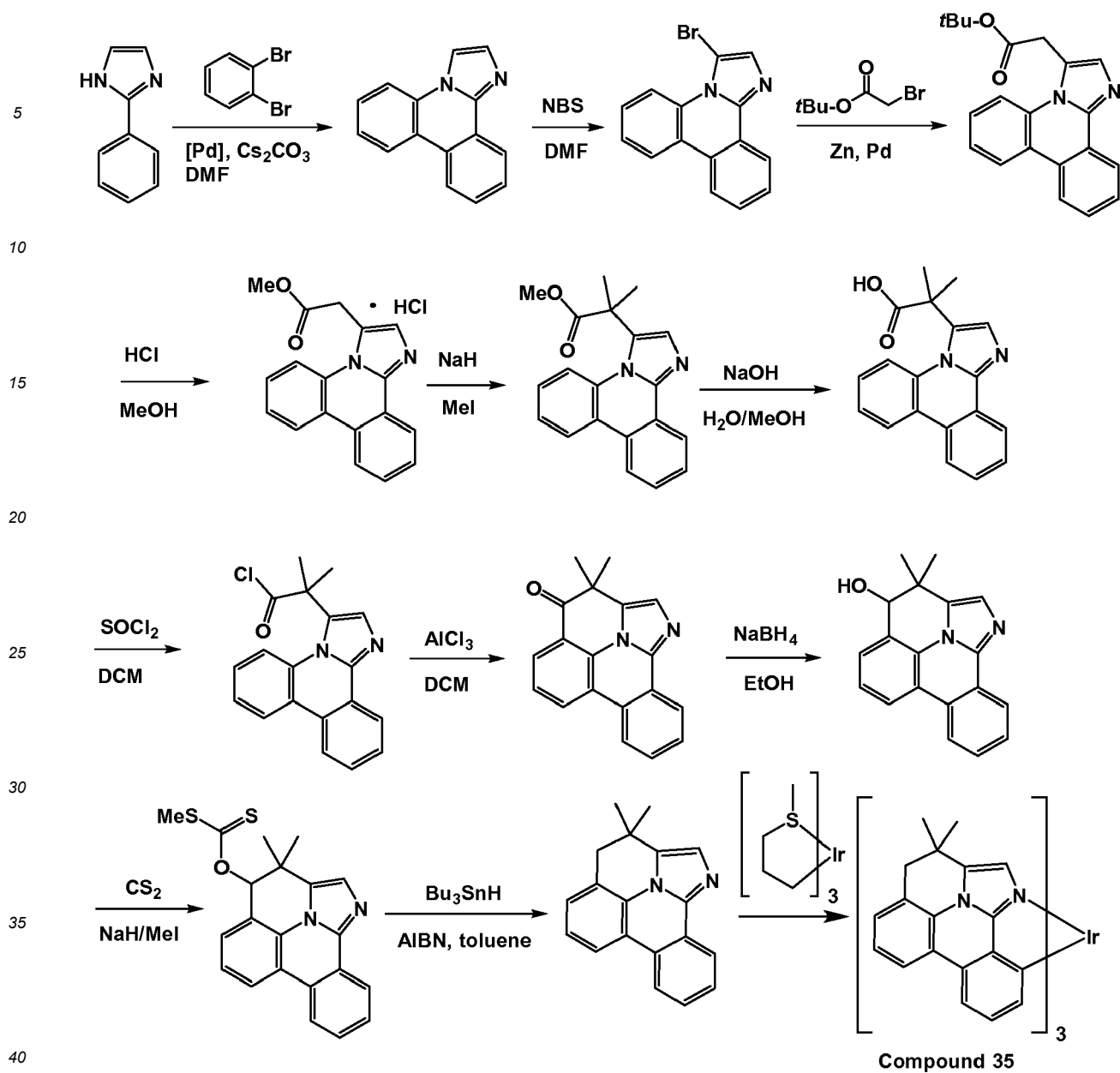
Scheme 5
