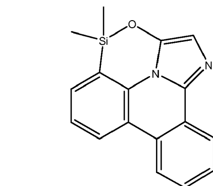
Compound (1-15)
