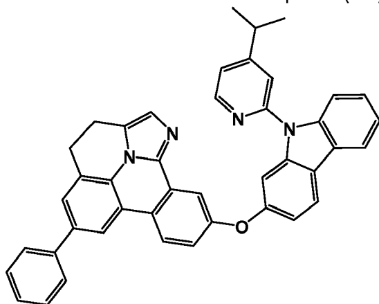
Compound (3-3)
