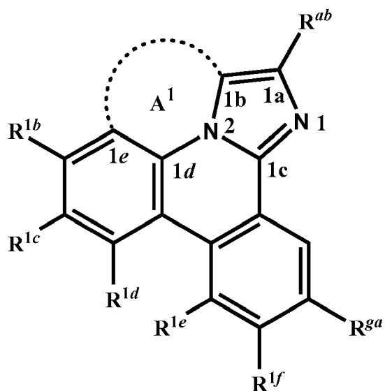
Formula (2a)
