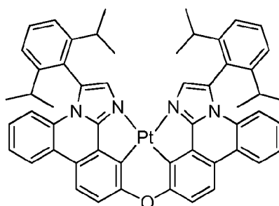
comparative compound 5
