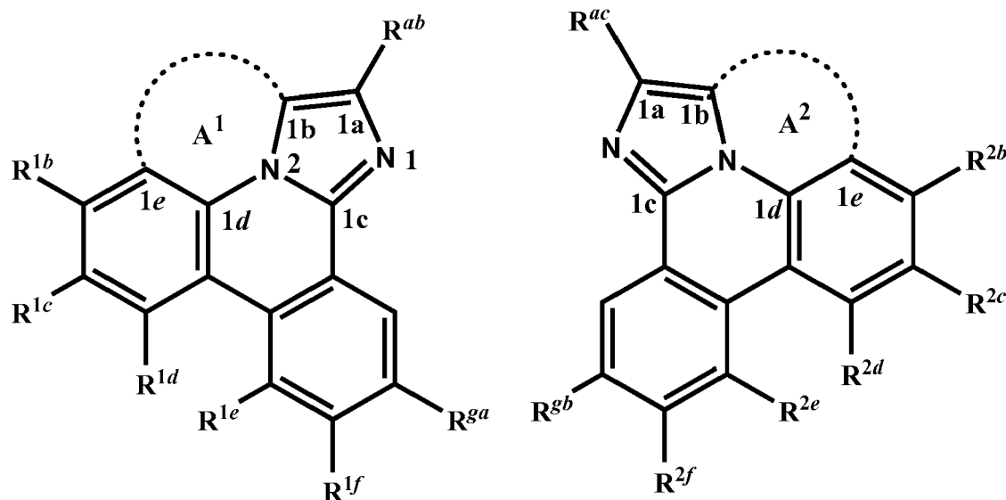
Formula (2a)
