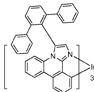
comparative compound 3
