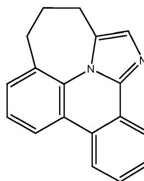
Compound (1-16)
