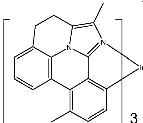
Compound 88
