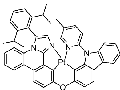
comparative compound 4
