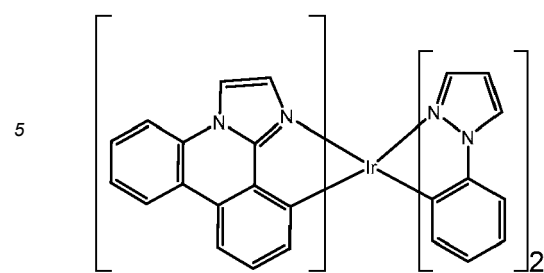
comparative compound 7
