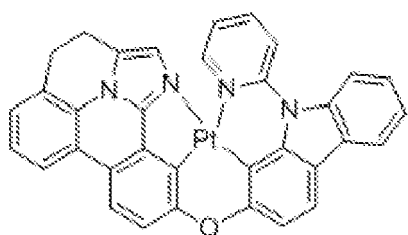
Compound 101
