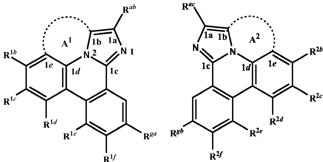
Formula (2a)
