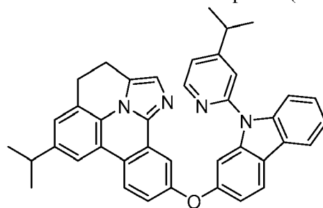
Compound (3-6)
