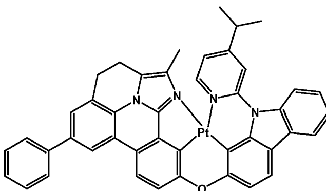
Compound 108
