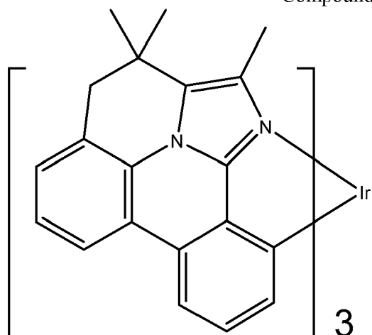
Compound 84
