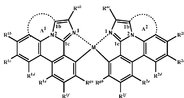
Formula (2)
