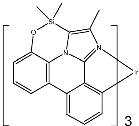
Compound 63
