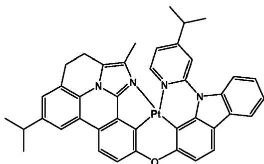
Compound 107
