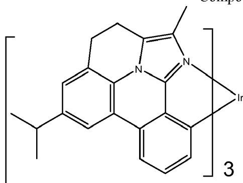
Compound 60
