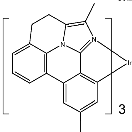
Compound 89
