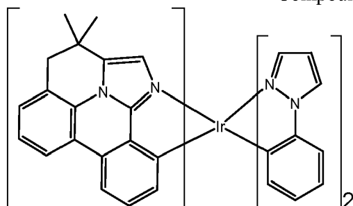
Compound 48
