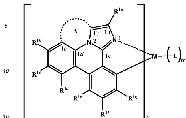
Formula (1)
