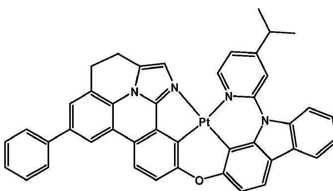
Compound 106
