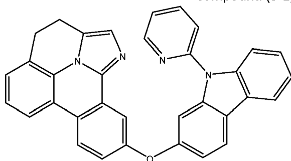
Compound (3-1)
