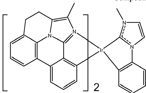
Compound 75
