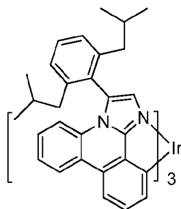
comparative compound 2
