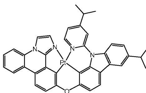
comparative compound 8
