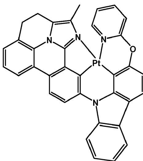
Compound 109
