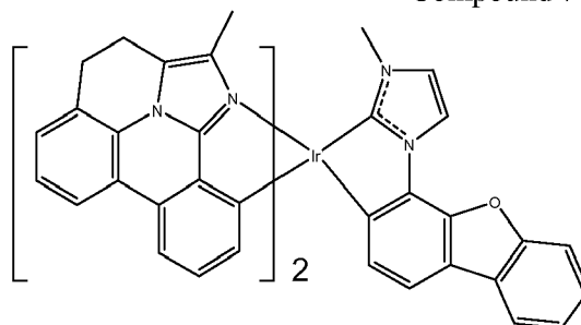
Compound 76
