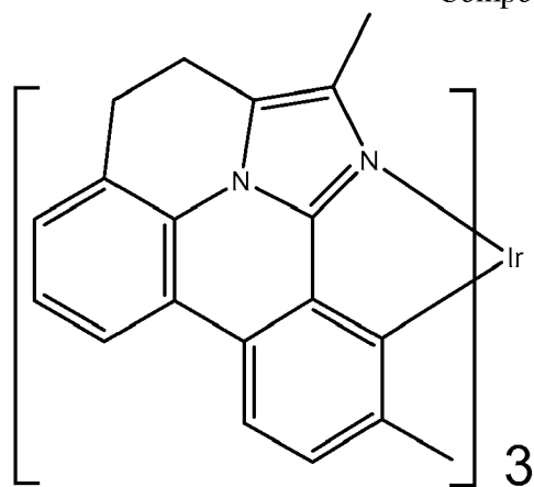
Compound 90
