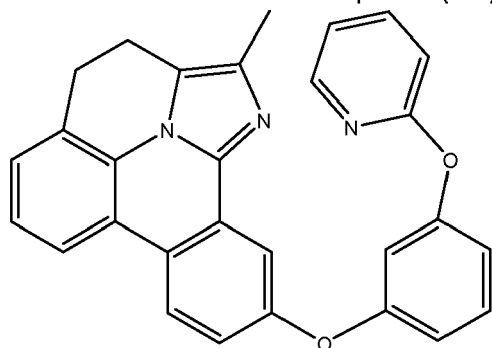
Compound (3-5)
