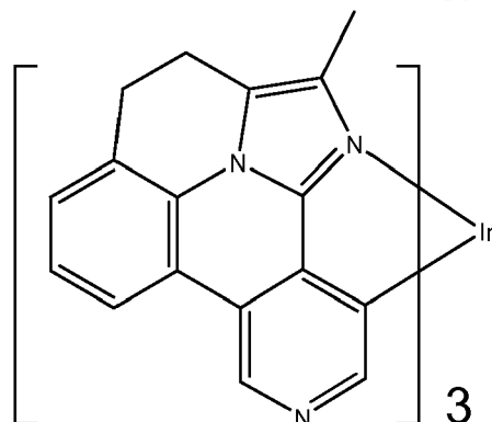
Compound 72
