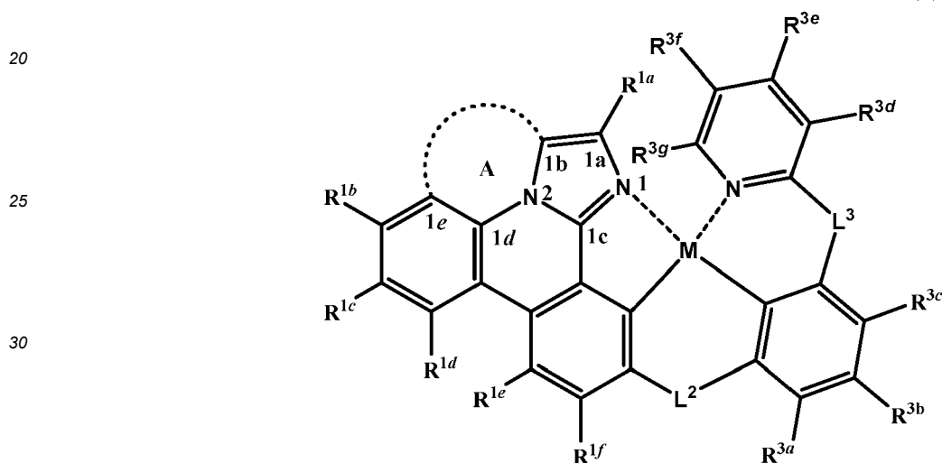
Formula (3)
