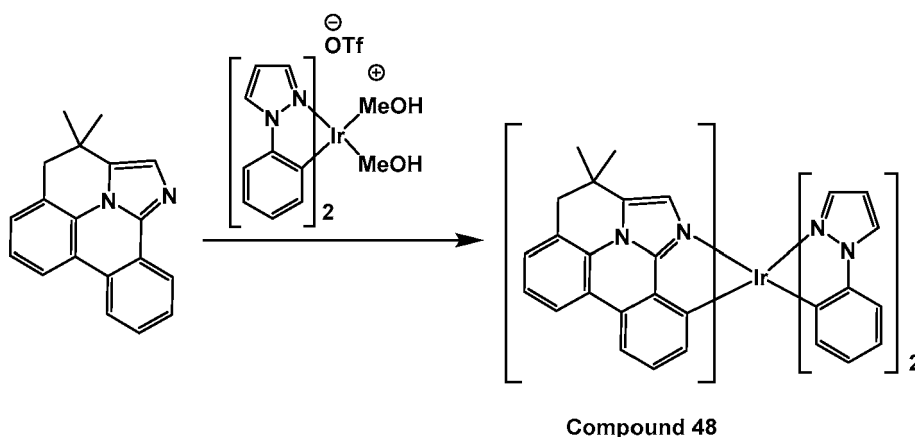
Scheme 6
