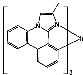
Comparative compound 6
