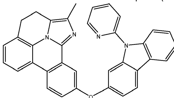
Compound (3-4)
