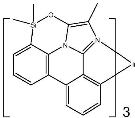
Compound 64
