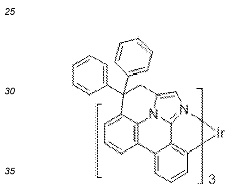
Compound 5
