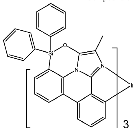
Compound 62
