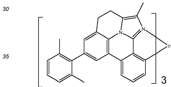
Compound 81
