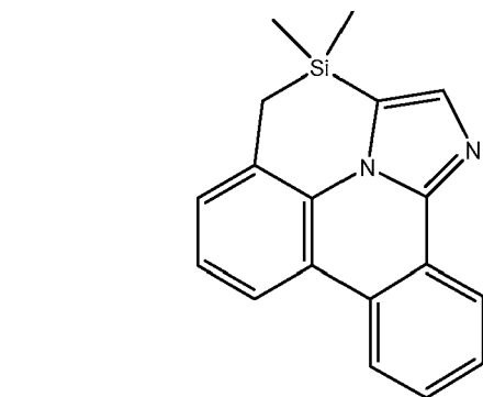
Compound (1-23)
