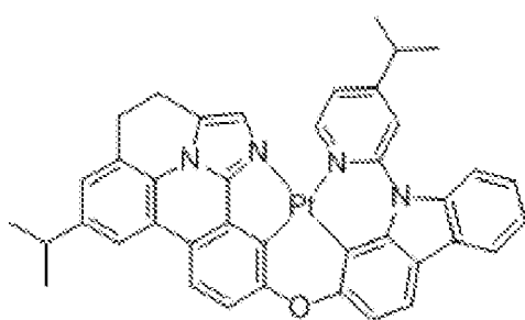
Compound 105
