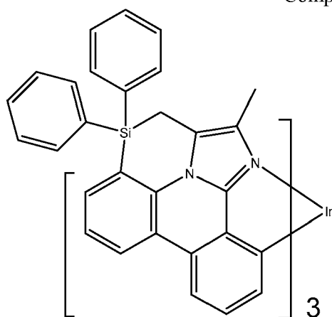
Compound 83
