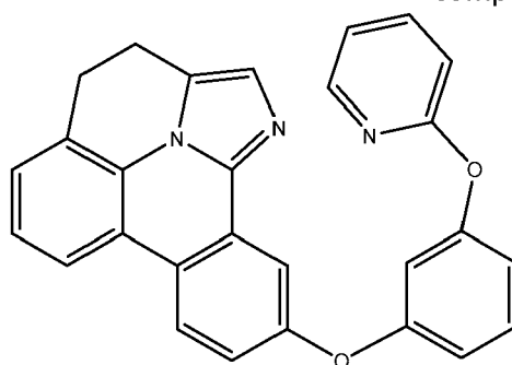
Compound (3-2)
