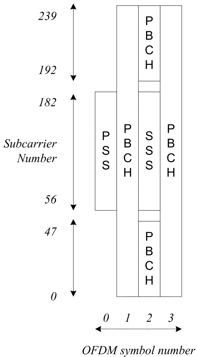
FIG. 5 (PRIOR ART)
