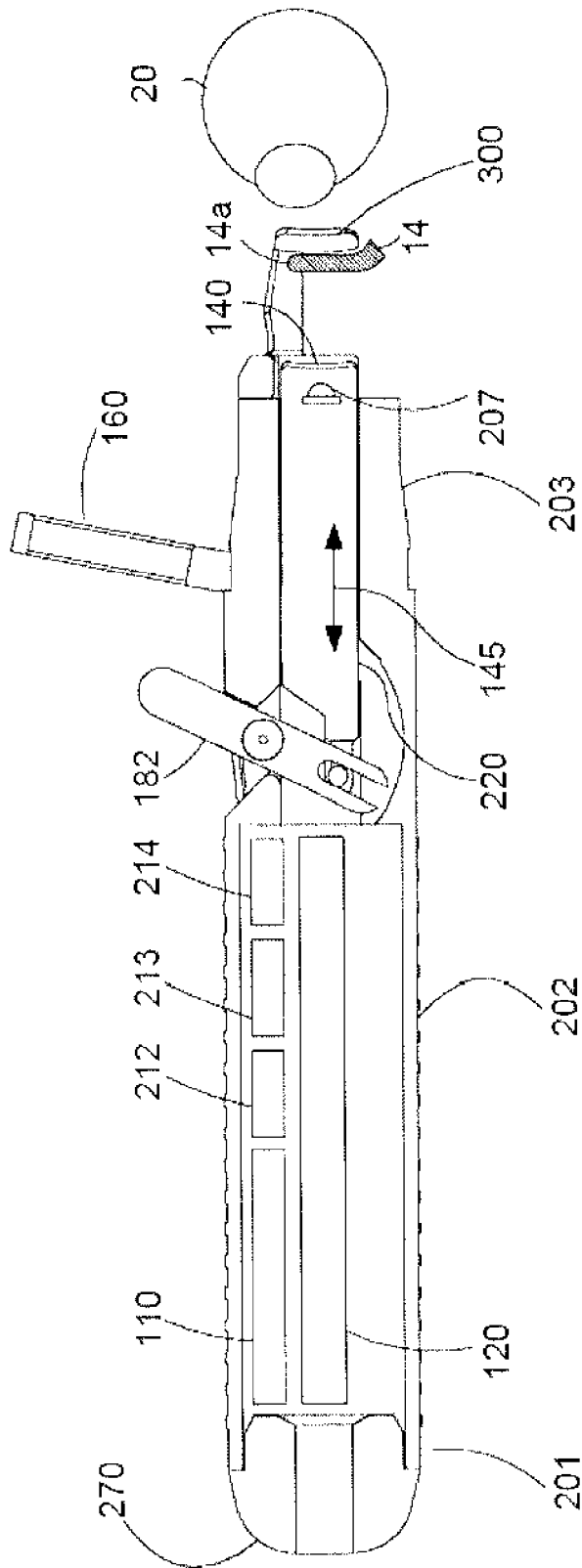
200 SECTION B-B FIGURE 15D
