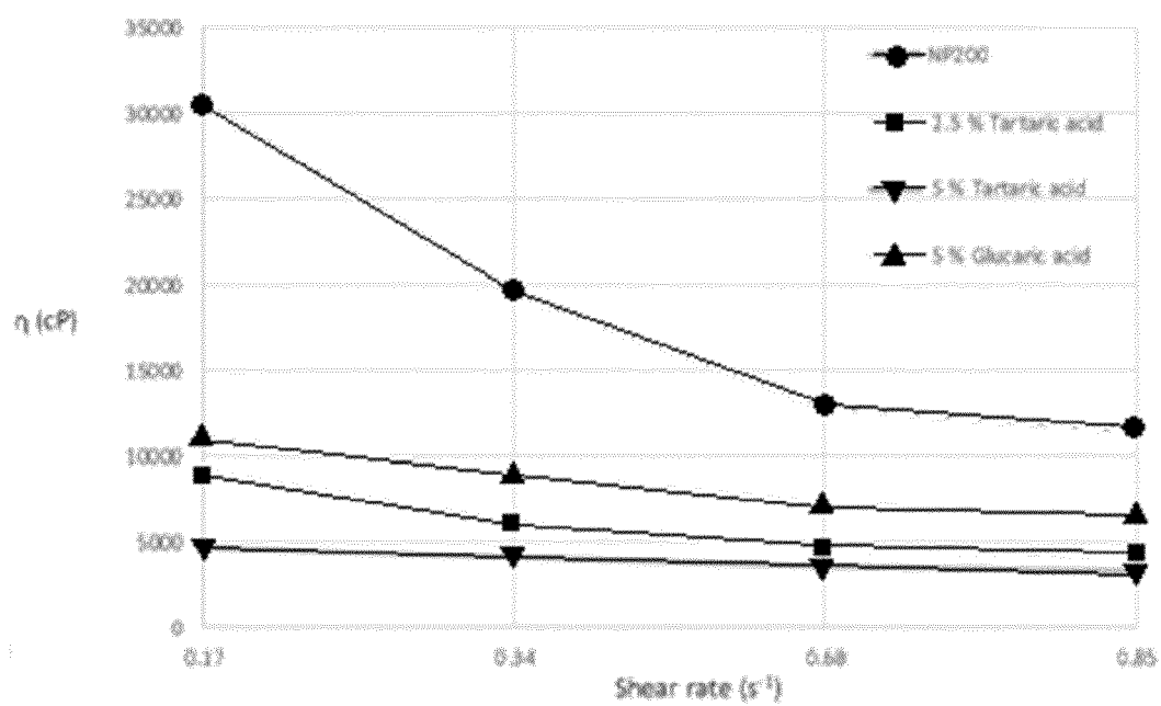
Viscosity vs shear rate for NP 200 and additives after 120 mins
