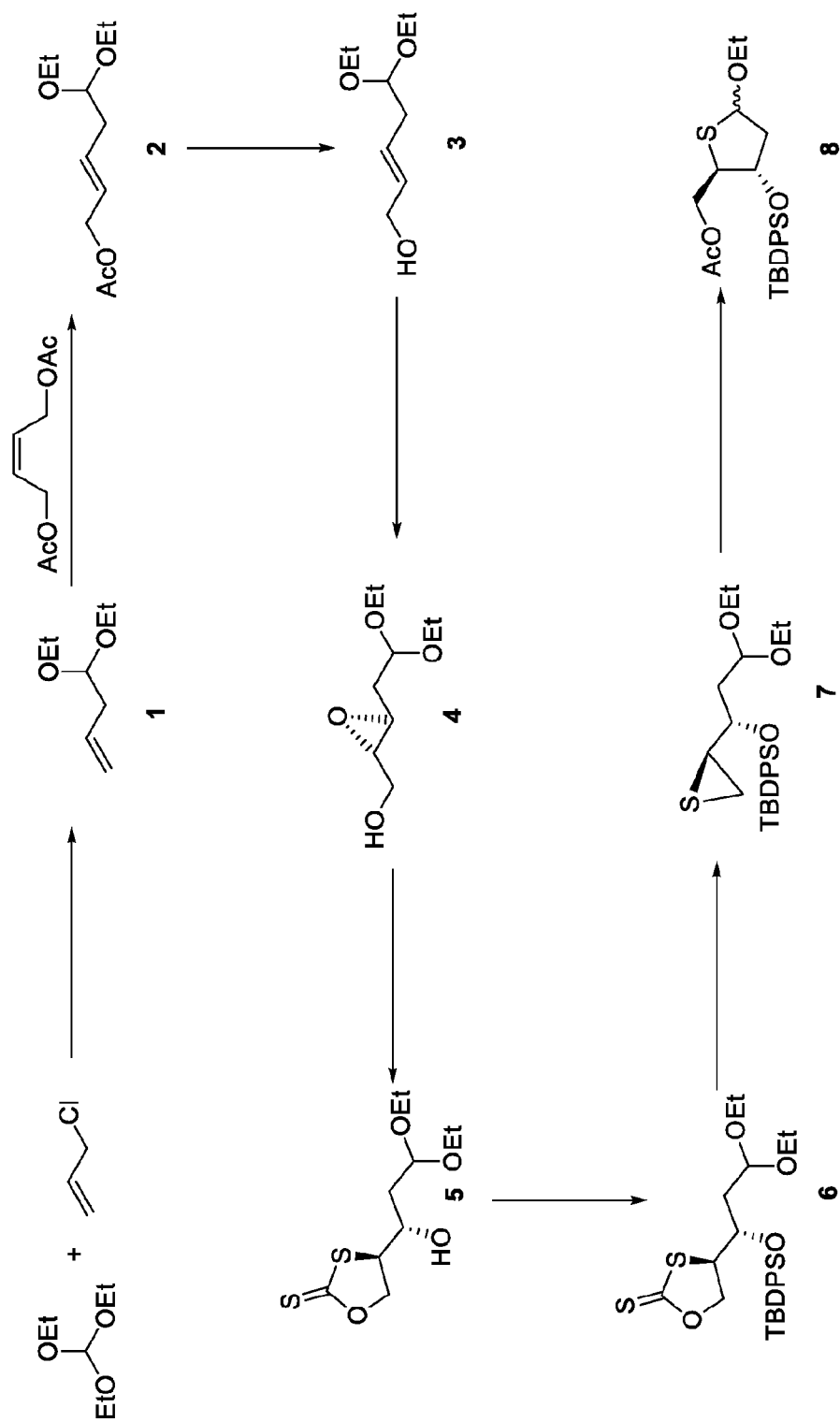
Scheme 2. Sugar Synthesis
