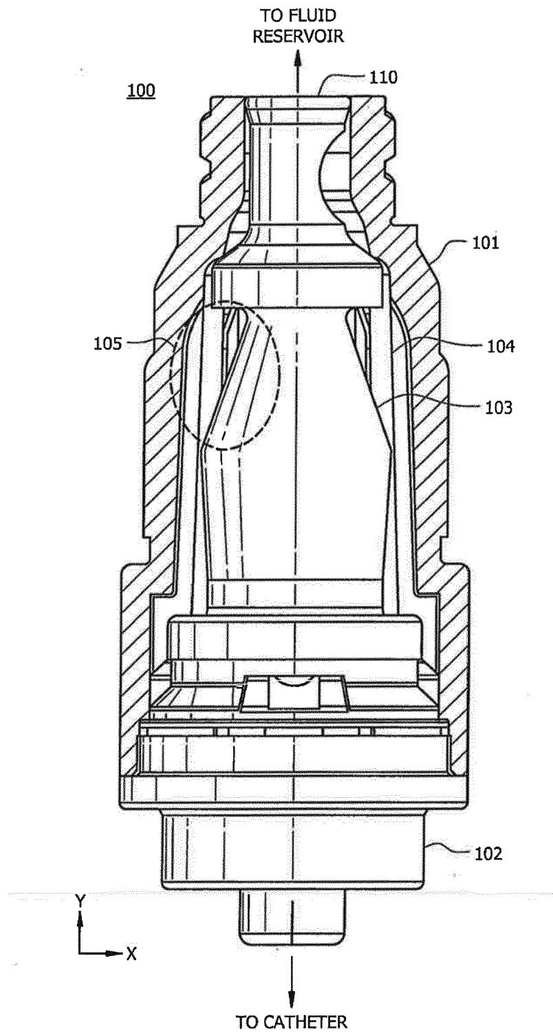
FIG. 1 (Prior Art)
