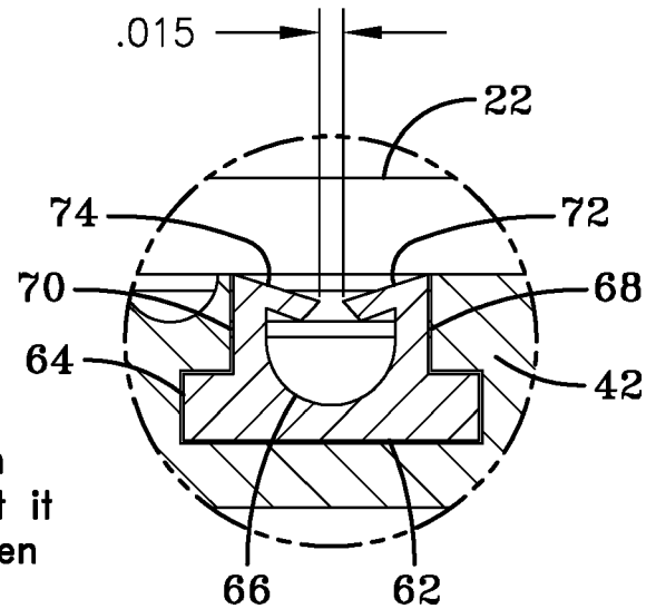
Detail B FIG-4
