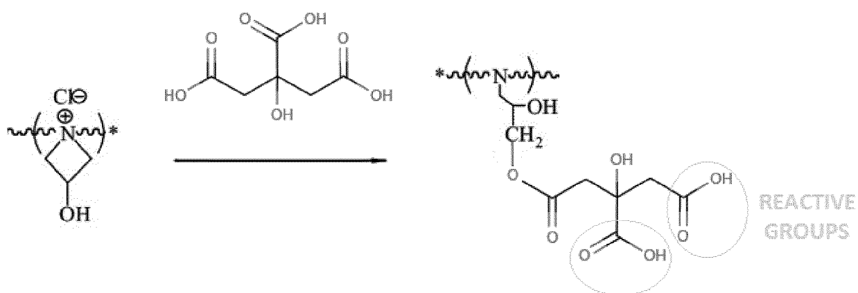
Figure 5. Polyamido-amine epichlorohydrin activation with Citric acid
