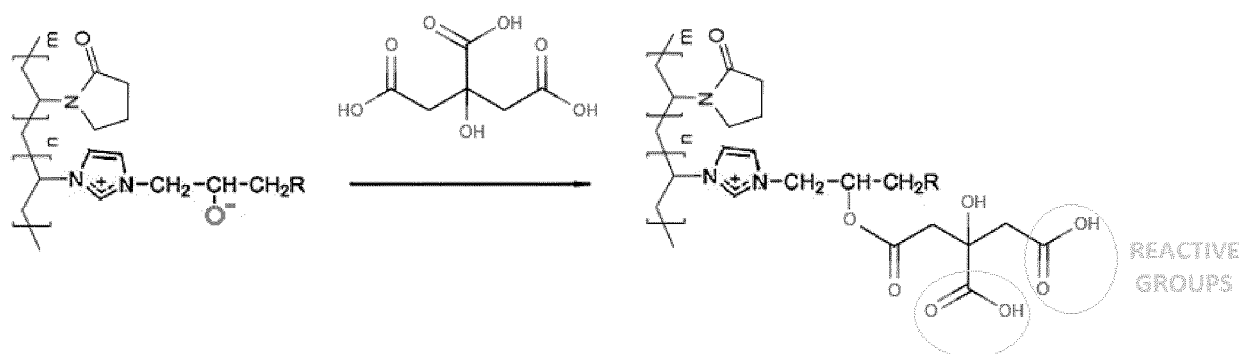
Figure 4. (Imidazole-Epichlorohydrin)-adduct activation with Citric acid
