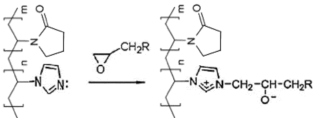
Figure 1. Stabilized cationic charge on a branched quaternary amine moiety.
