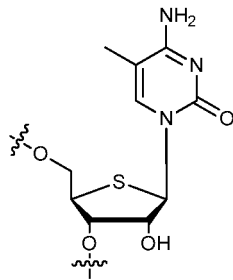
4'Thio-5-Methyl-Cytidine
