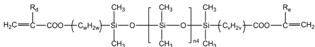
[Chemical Formula2d]
