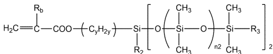
[Chemical Formula2c]
