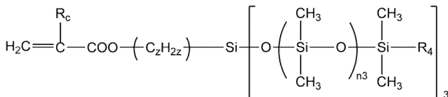
[Chemical Formula2d]
