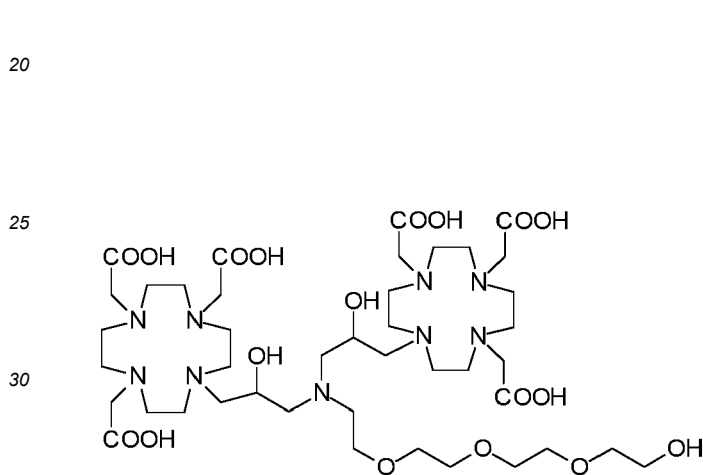
Compound 7
