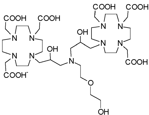
Compound 4
