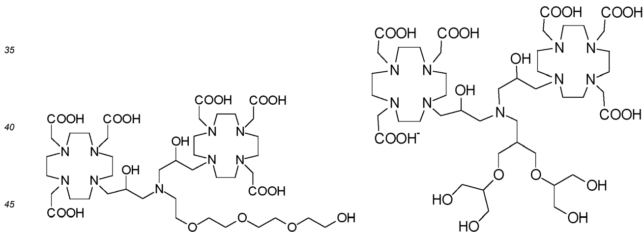
Compound 5
