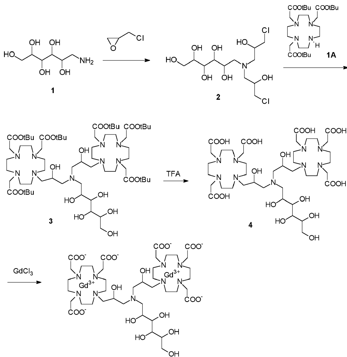
Scheme 5
