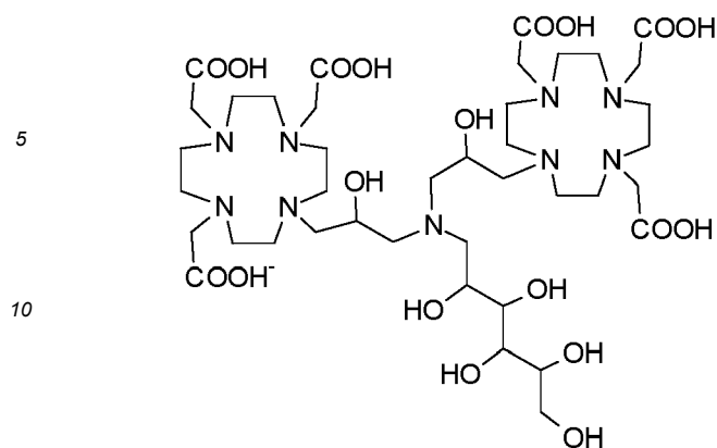
Compound 3
