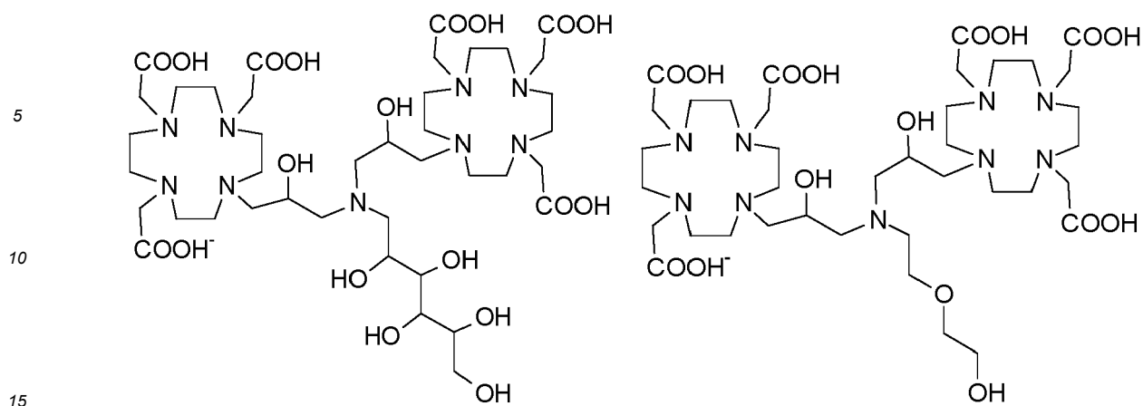
Compound 3
