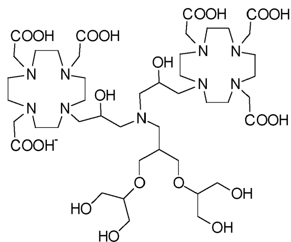
Compound 8
