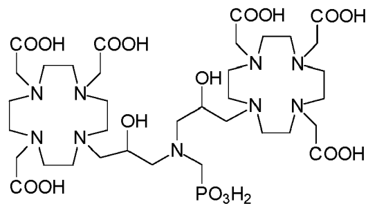
Compound 2
