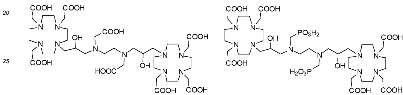
Compound 5
