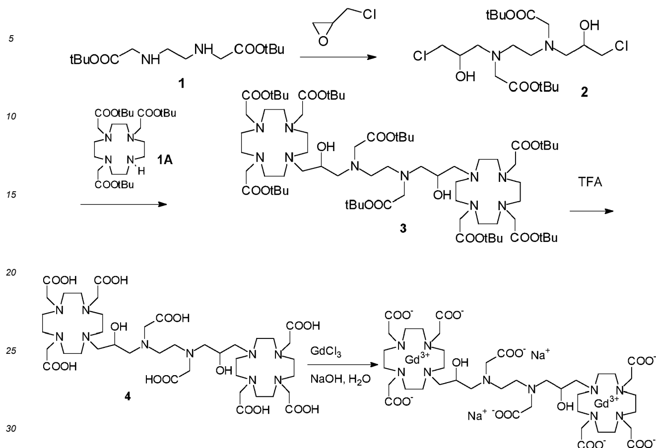
Scheme 6
