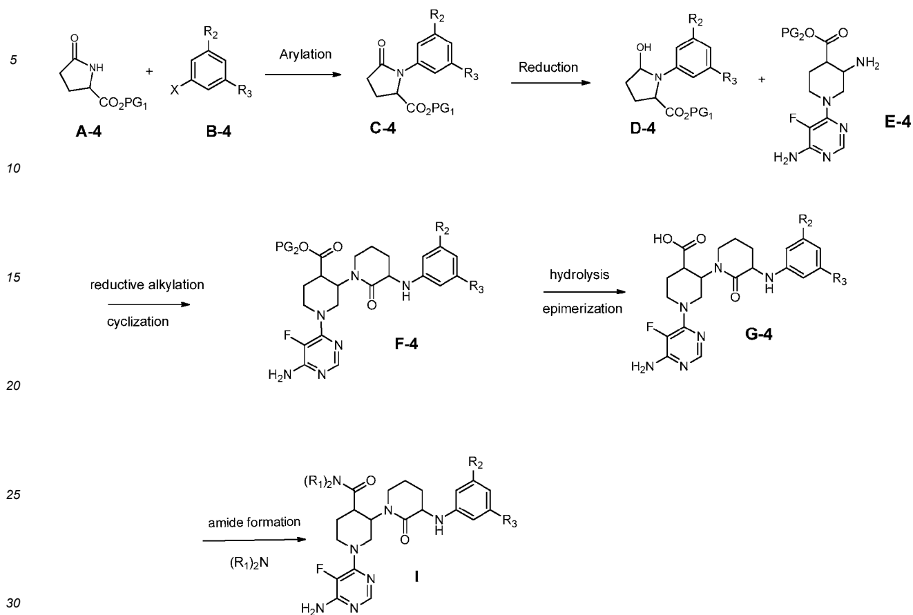
Scheme 4
