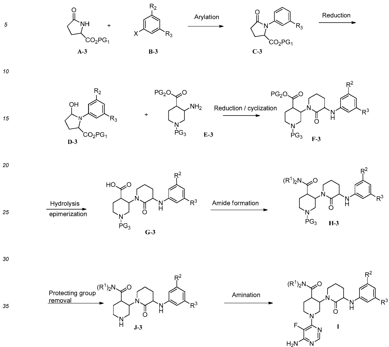
Scheme 3
