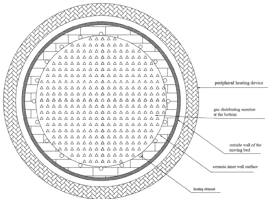
top view of the cross-section
