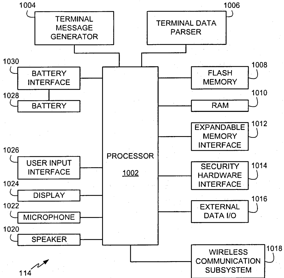
WIRELESS TERMINAL
