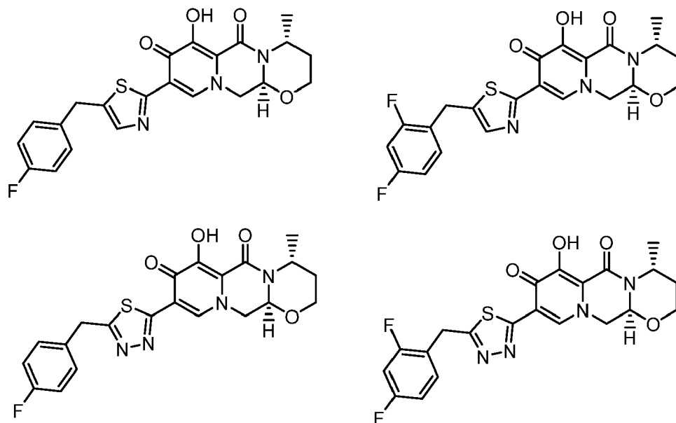
[Chemical Formula 2]
