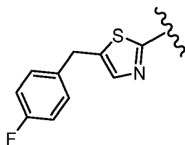
[Chemical Formula 22]
