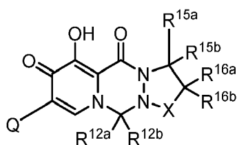
[Chemical Formula 17]
