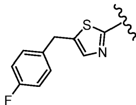
[Chemical Formula 2 2]
