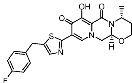
[Chemical Formula 2]
