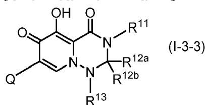
[Chemical Formula 44]
