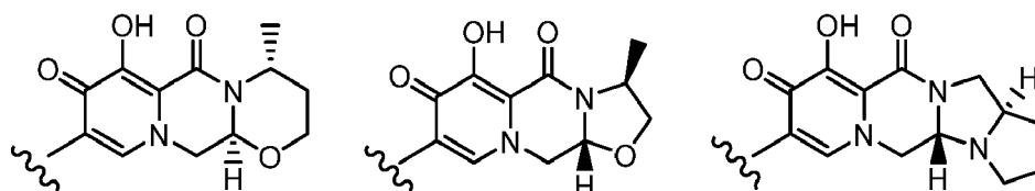
[Chemical Formula 28]
