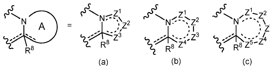
[Chemical Formula 4]
