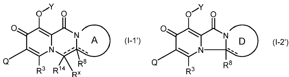
[Chemical Formula 24]
