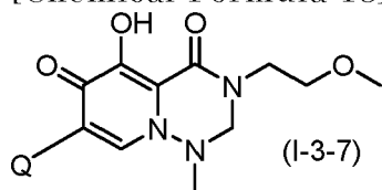
[Chemical Formula 18]
