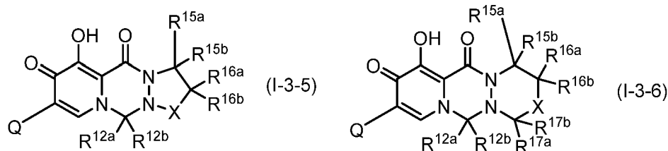
[Chemical Formula 46]
