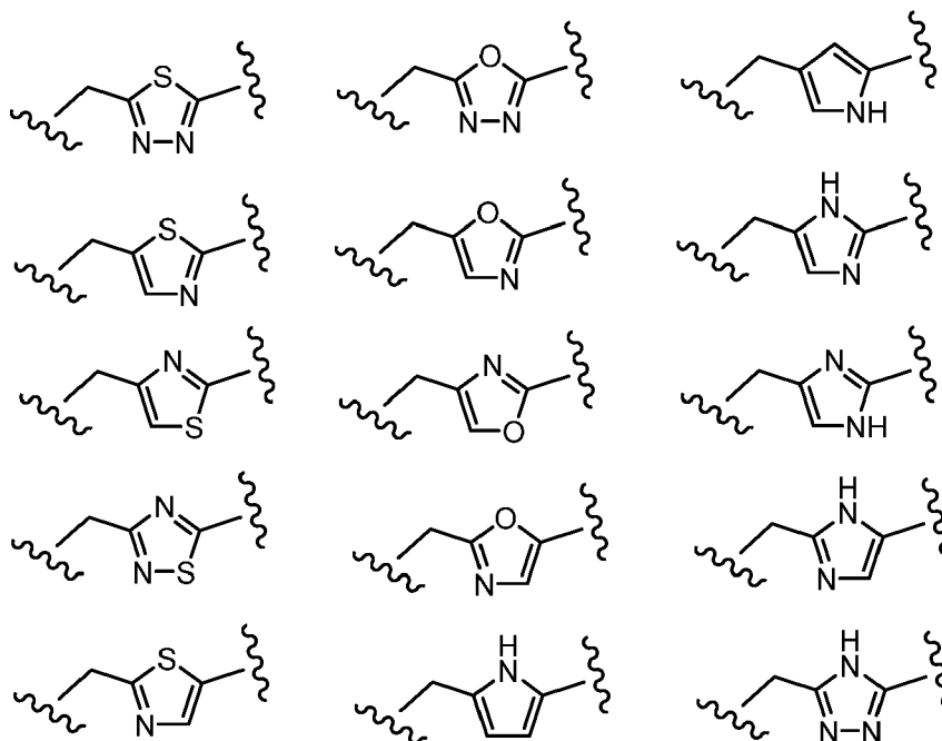
[Chemical Formula 27]
