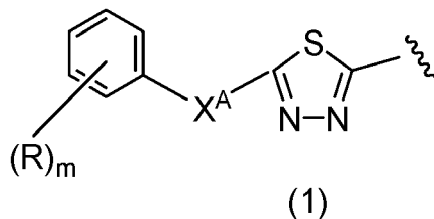
[Chemical Formula 21]
