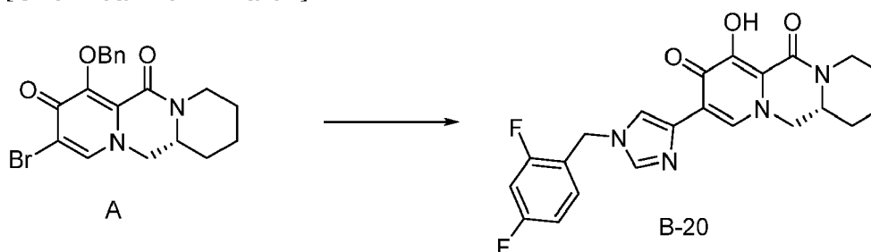
[Chemical Formula 64]
