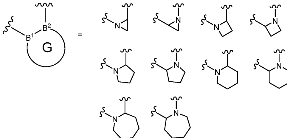
[Chemical Formula 15]
