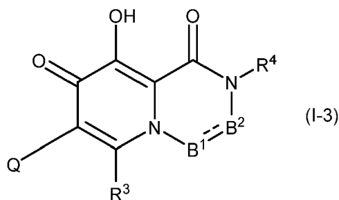
[Chemical Formula 10]
