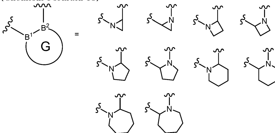
[Chemical Formula 15]
