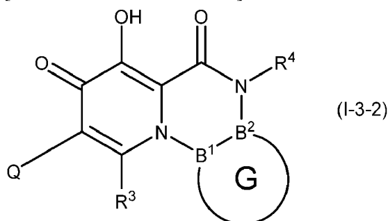
[Chemical Formula 42]
