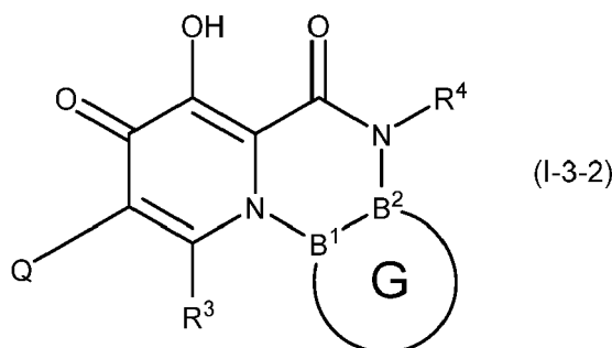
[Chemical Formula 1 4]
