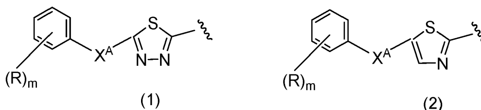
[Chemical Formula 21]
