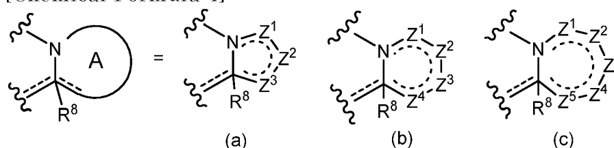
[Chemical Formula 4]
