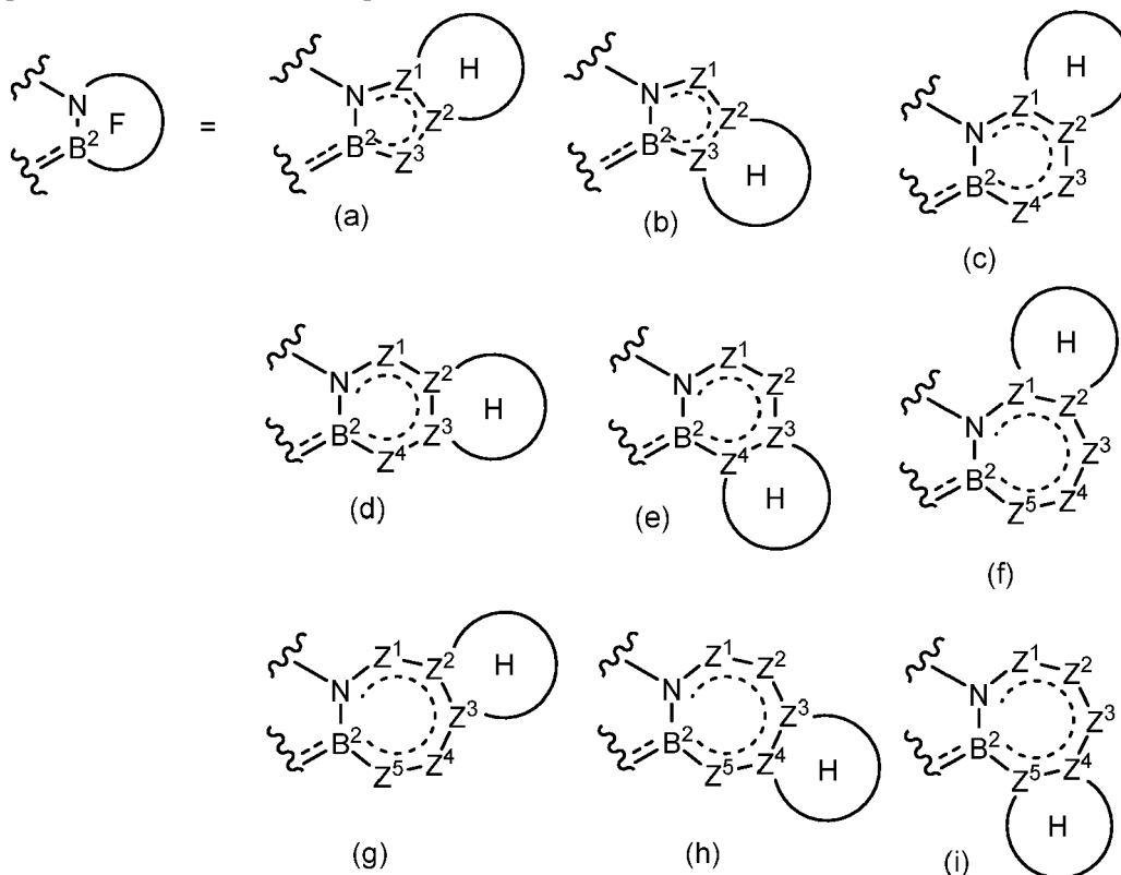
[Chemical Formula 41]
