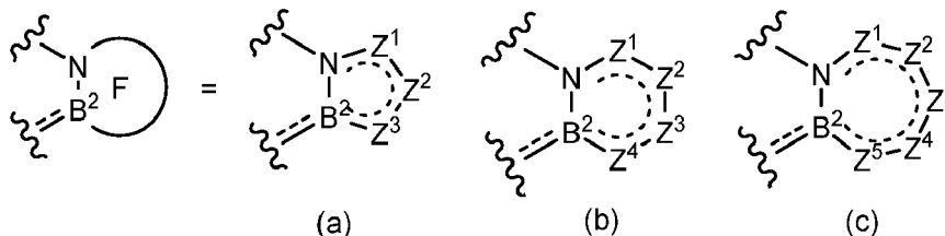
[Chemical Formula 12]
