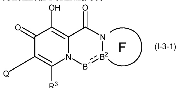
[Chemical Formula 39]
