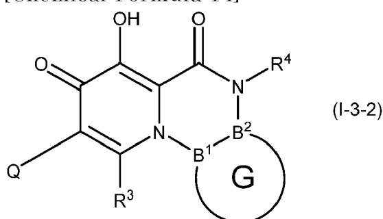
[Chemical Formula 14]
