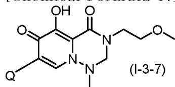
[Chemical Formula 47]
