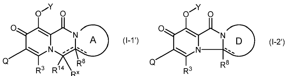
[Chemical Formula 49]
