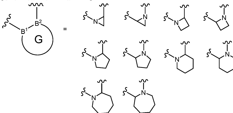
[Chemical Formula 1 5]
