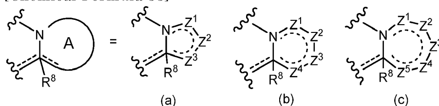
[Chemical Formula 33]
