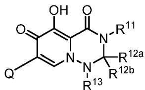
[Chemical Formula 16]
