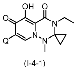
[Chemical Formula 48]
