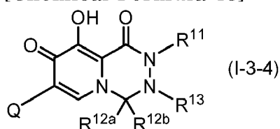
[Chemical Formula 45]
