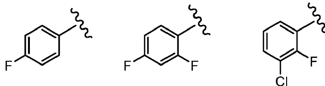
[Chemical Formula 26]
