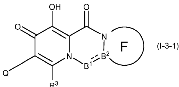
[Chemical Formula 11]
