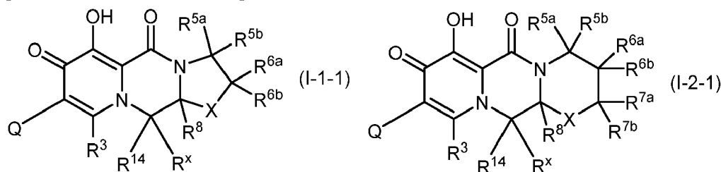
[Chemical Formula 35]
