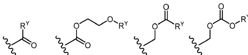
[Chemical Formula 50]
