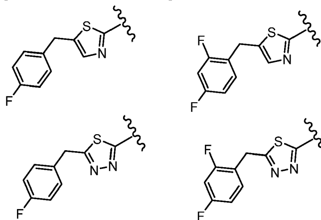
[Chemical Formula 22]
