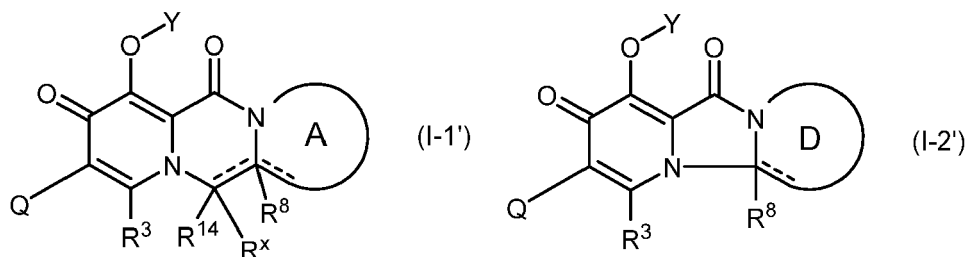
[Chemical Formula 2 4]
