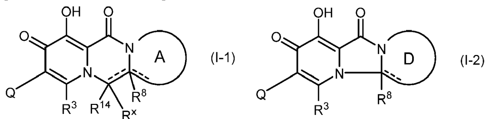
[Chemical Formula 1]
