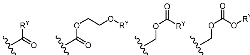
[Chemical Formula 25]
