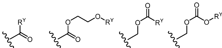
[Chemical Formula 2 5]
