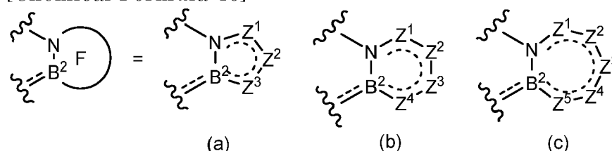
[Chemical Formula 40]
