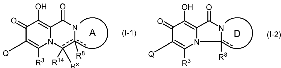
[Chemical Formula 32]
