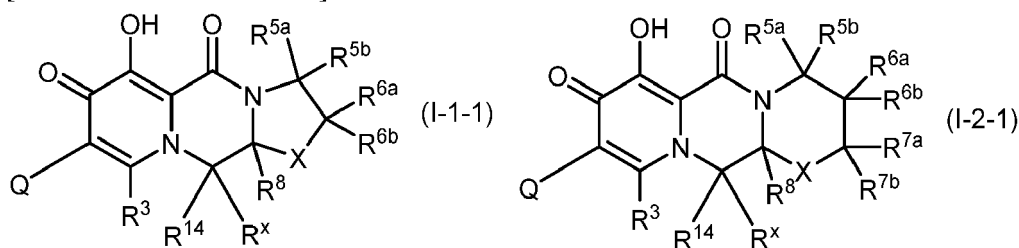
[Chemical Formula 6]
