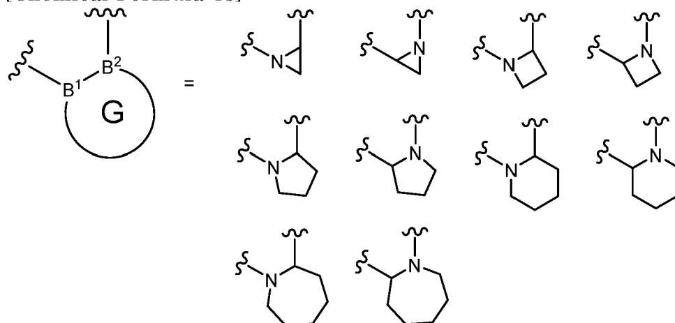
[Chemical Formula 43]
