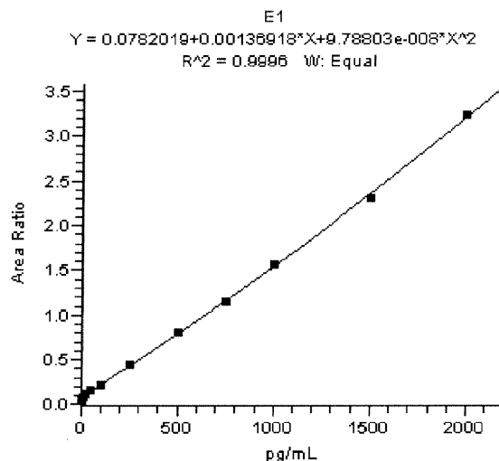
Figure 1. Linearity – Typical Calibration Curve
