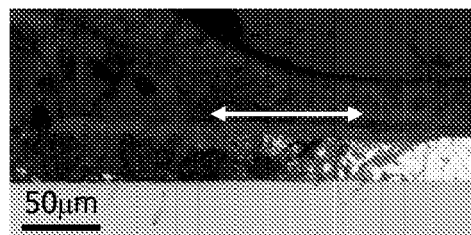
Figure 4: Example of the more narrow and uniform corrosion front for metallic coated steel strip in accordance with the present invention, under paint in a marine environment.
