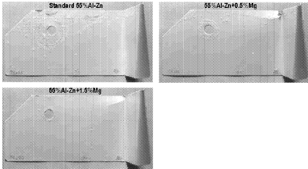
Figure 2 Improved corrosion performance for fluorocarbon painted, metallic coated steel strip in accordance with the present invention, for unwashed exposure in a severe marine environment.
