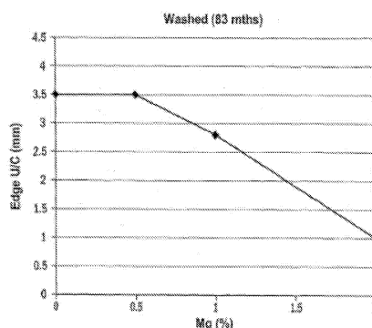
Figure 1: Reduction in the level of edge undercutting for painted, metallic coated steel strip in accordance with the present invention, for washed exposure in a severe marine environment.
