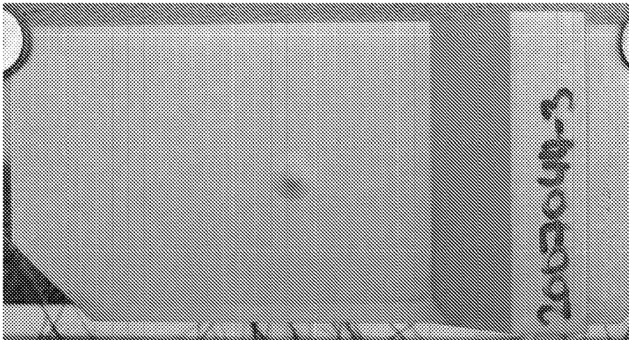
Figure 7: No red rust staining on the Al/Zn metallic coated steel strip in accordance with the present invention (total coating mass of 100\text{g/m}^2 of coating), exposed in a severe "acid rain" environment for 6 months.
