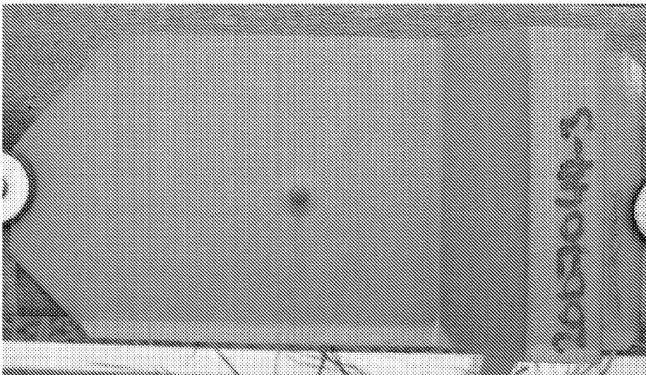
Figure 9: No red rust staining on the Al/Zn metallic coated steel strip in accordance with the present invention (total coating mass of 100g/m 2 of coating), exposed in a severe "acid rain" environment for 18 months.
