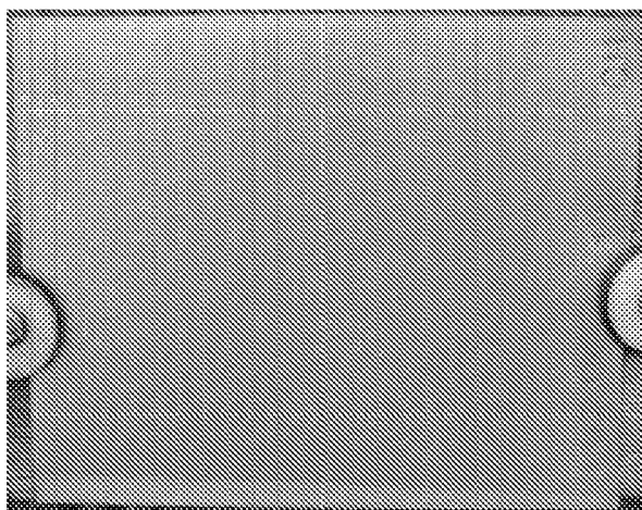
Figure 11: No red rust staining on the Al/Zn metallic coated steel strip in accordance with the present invention, with columnar structure (total coating mass of 50\text{g/m}^2 of coating), exposed in a severe "acid rain" environment for 4 months.
