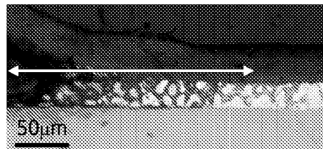
Figure 3: Example of the extensive corrosion front for a conventional Al/Zn coating under paint in a marine environment.
