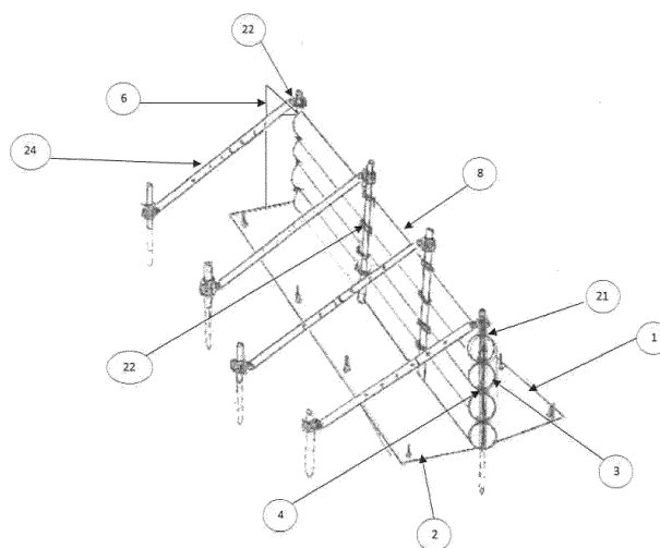
Figure 5 – Deployed Barrier - Rear Isometric View
