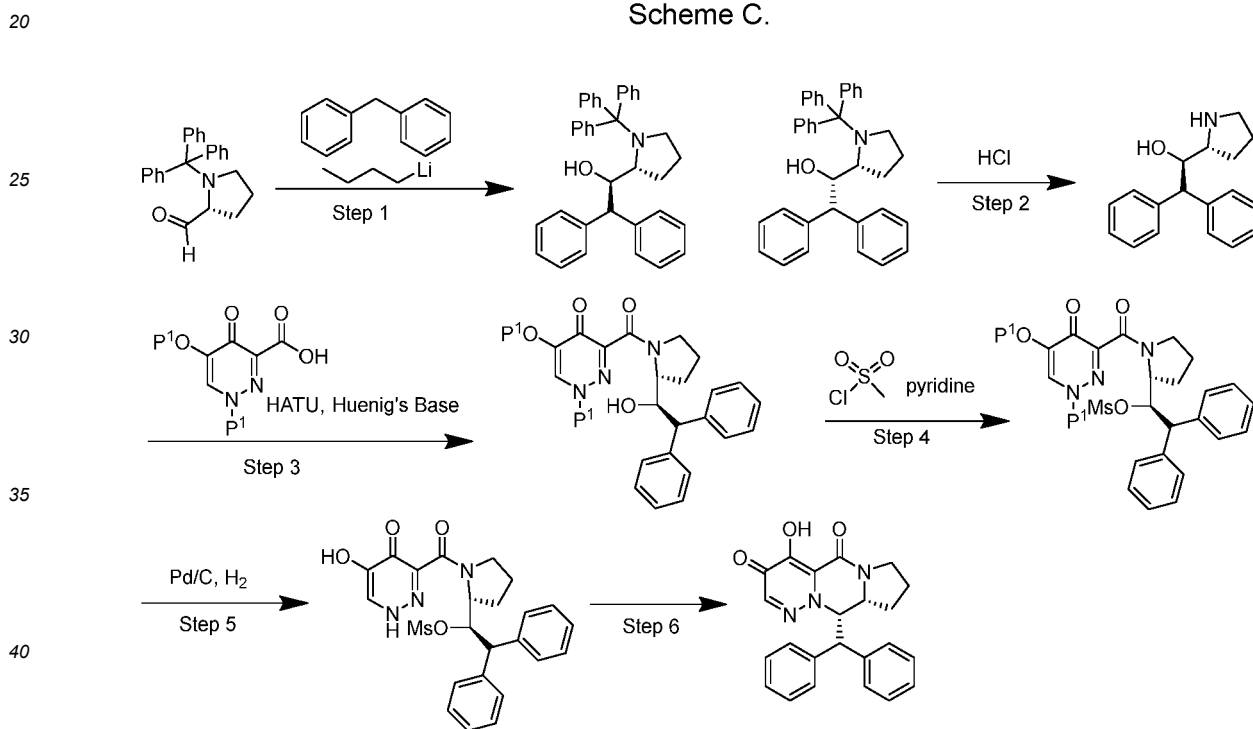
Scheme C.
