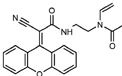
2-cyano-N-(2-(N-vinylacetamido)ethyl)-2-(9H-xanthen-9-ylidene)acetamide
