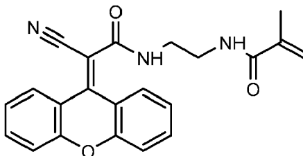
N-(2-(2-cyano-2-(9H-xanthen-9-ylidene)acetamido)ethyl)methacrylamide
