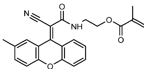
(E)-2-(2-cyano-2-(2-methyl-9H-xanthen-9-ylidene)acetamido)ethyl methacrylate
