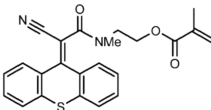
2-(2-cyano-N-methyl-2-(9H-thioxanthen-9-ylidene)acetamido)ethyl methacrylate
