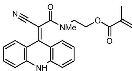
2-(2-(acridin-9(10H)-ylidene)-2-cyano-N-methylacetamido)ethyl methacrylate
