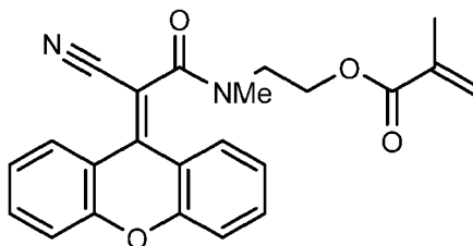
2-(2-cyano-N-methyl-2-(9H-xanthen-9-ylidene)acetamido)ethyl methacrylate
