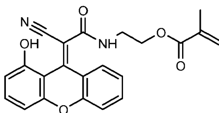
(E)-2-(2-cyano-2-(1-hydroxy-9H-xanthen-9-ylidene)acetamido)ethyl methacrylate
