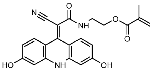
2-(2-cyano-2-(3,6-dihydroxyacrididin-9(10H)-ylidene)acetamido)ethyl methacrylate
