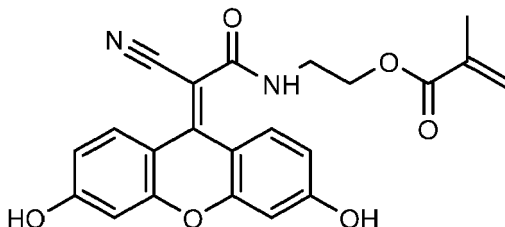
2-(2-cyano-2-(3,6-dihydroxy-9H-xanthen-9-ylidene)acetamido)ethyl methacrylate
