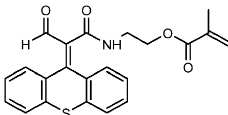
2-(3-oxo-2-(9H-thioxanthen-9-ylidene)propanamido)ethyl methacrylate
