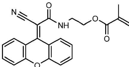
2-(2-cyano-2-(9H-xanthen-9-ylidene)acetamido)ethyl methacrylate
