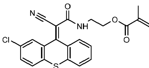
(E)-2-(2-(2-chloro-9H-thioxanthen-9-ylidene)-2-cyanoacetamido)ethyl methacrylate
