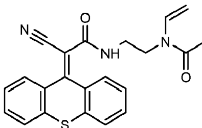
2-cyano-2-(9H-thioxanthen-9-ylidene)-N-(2-(N-vinylacetamido)ethyl)acetamide
