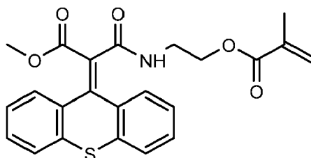
2-(3-methoxy-3-oxo-2-(9H-thioxanthen-9-ylidene)propanamido)ethyl methacrylate
