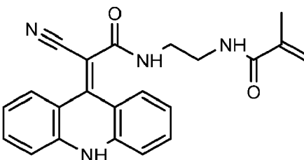
N-(2-(2-(acridin-9(10H)-ylidene)-2-cyanoacetamido)ethyl)methacrylamide
