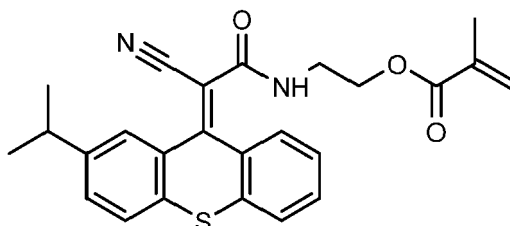
(E)-2-(2-cyano-2-(2-isopropyl-9H-thioxanthen-9-ylidene)acetamido)ethyl methacrylate
