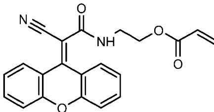
2-(2-cyano-2-(9H-xanthen-9-ylidene)acetamido)ethyl acrylate
