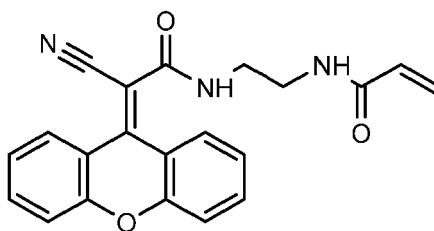
N-(2-(2-cyano-2-(9H-xanthen-9-ylidene)acetamido)ethyl)acrylamide
