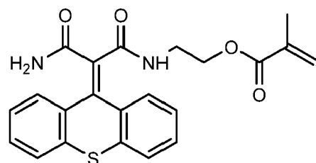
2-(3-amino-3-oxo-2-(9H-thioxanthen-9-ylidene)propanamido)ethyl methacrylate
