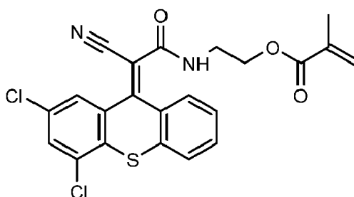
(E)-2-(2-cyano-2-(2,4-dichloro-9H-thioxanthen-9-ylidene)acetamido)ethyl methacrylate
