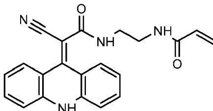
N-(2-(2-(acridin-9(10H)-ylidene)-2-cyanoacetamido)ethyl)acrylamide
