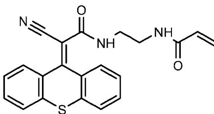
N-(2-(2-cyano-2-(9H-thioxanthen-9-ylidene)acetamido)ethyl)acrylamide
