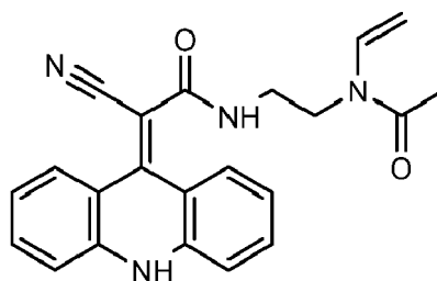
2-(acridin-9(10H)-ylidene)-2-cyano-N-(2-(N-vinylacetamido)ethyl)acetamide
