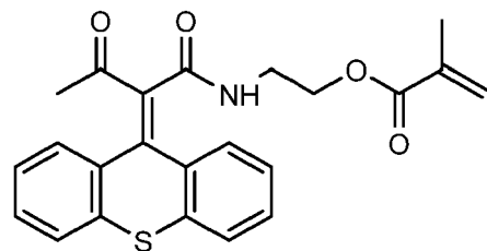
2-(3-oxo-2-(9H-thioxanthen-9-ylidene)butanamido)ethyl methacrylate
