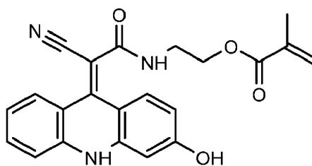
(Z)-2-(2-cyano-2-(3-hydroxyacridin-9(10H)-ylidene)acetamido)ethyl methacrylate
