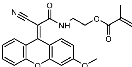
(Z)-2-(2-cyano-2-(3-methoxy-9H-xanthen-9-ylidene)acetamido)ethyl methacrylate
