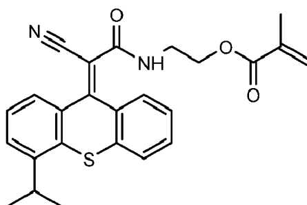
(E)-2-(2-cyano-2-(4-isopropyl-9H-thioxanthen-9-ylidene)acetamido)ethyl methacrylate
