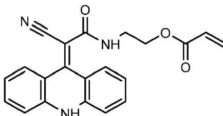
2-(2-(acridin-9(10H)-ylidene)-2-cyanoacetamido)ethyl acrylate
