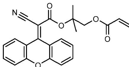
2-(2-cyano-2-(9H-xanthen-9-ylidene)acetoxy)-2-methylpropyl acrylate
