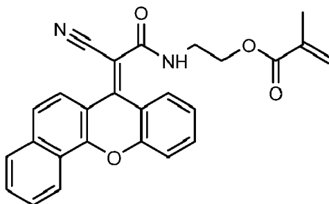
(E)-2-(2-(7H-benzo[c]xanthen-7-ylidene)-2-cyanoacetamido)ethyl methacrylate
