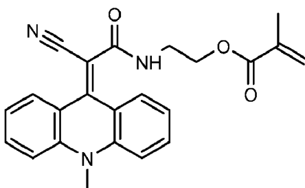
2-(2-cyano-2-(10-methylacrididin-9(10H)-ylidene)acetamido)ethyl methacrylate
