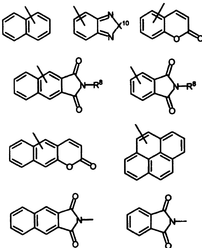
[Chem. 17]
