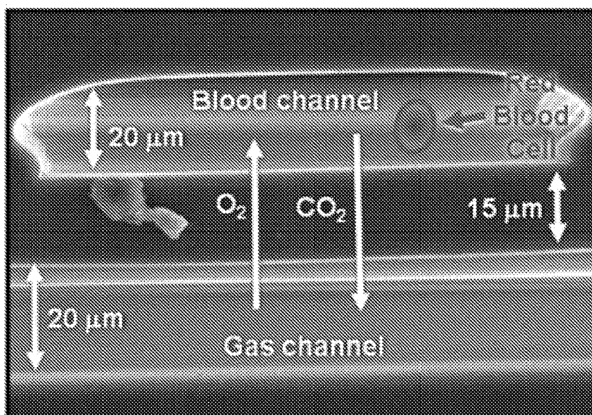
Microchannel Artificial Lung
