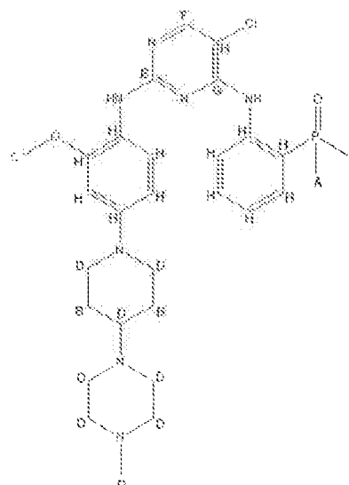
13 C-NMR Assignments
