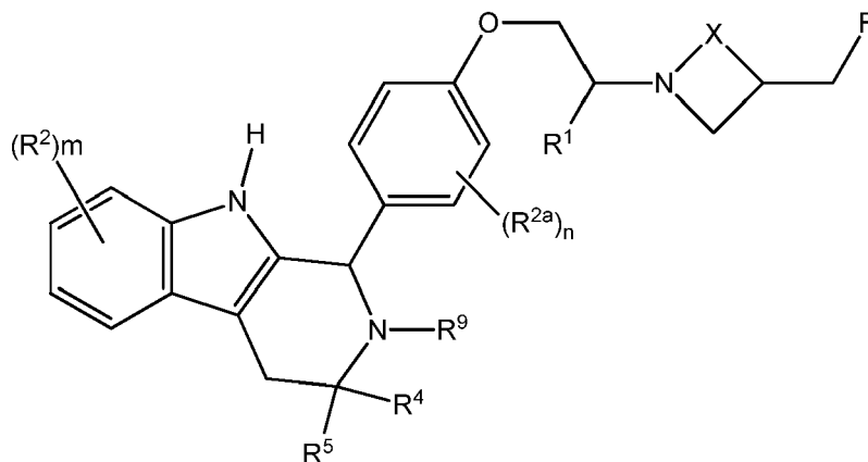
Formula (XIa);
