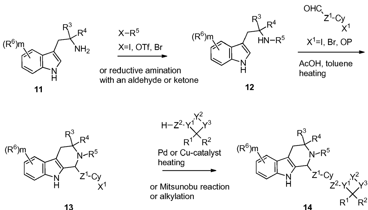
Scheme 3:
