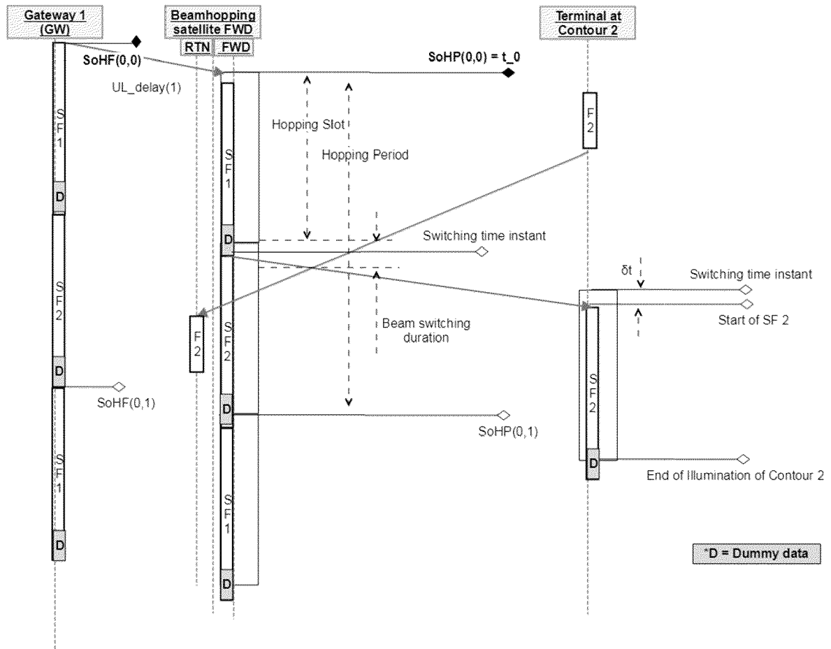
Beamhopping timeline
