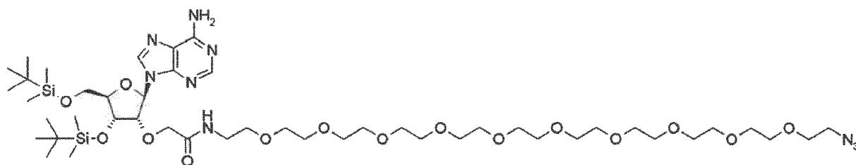
[Compound 10]
