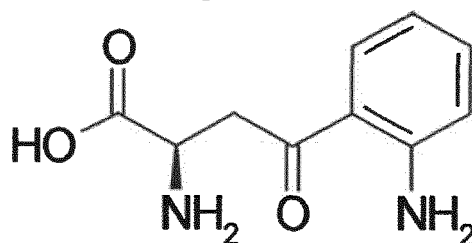
[Compound 19]
