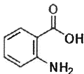
[Compound 2]
