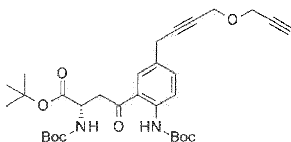
[Compound 39]
