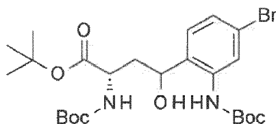
[Compound 28]
