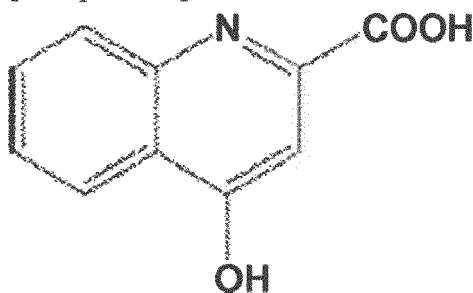
[Compound 4]
