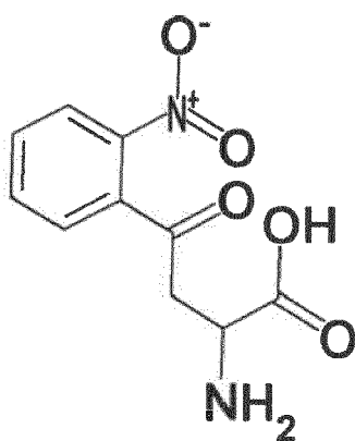
[Compound 24]
