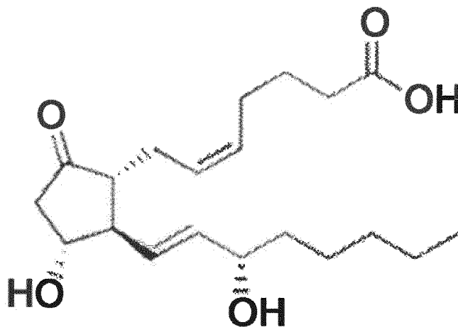
[Compound 5]
