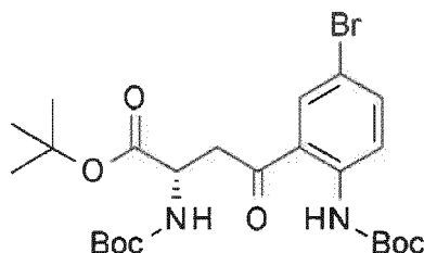
[Compound 37]
