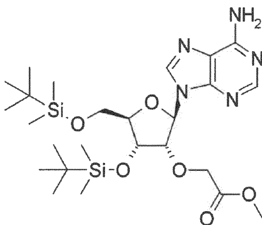
[Compound 8]
