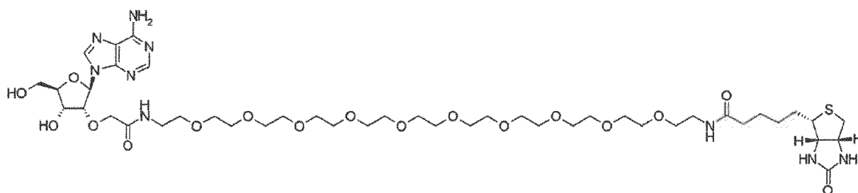
[Compound 18]
