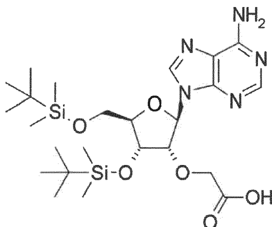
[Compound 9]
