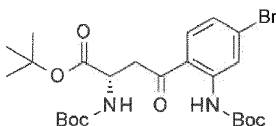
[Compound 29]
