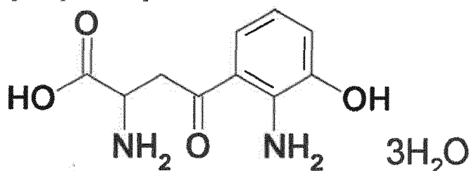
[Compound 20]
