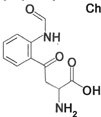
[Compound 22]
