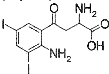
[Compound 23]
