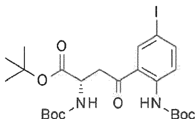
[Compound 38]
