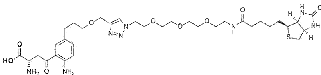
[Compound 41]
