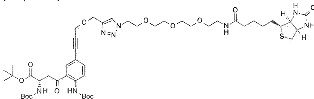
[Compound 40]
