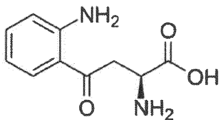
[Compound 1]
