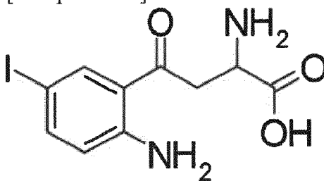
[Compound 25]
