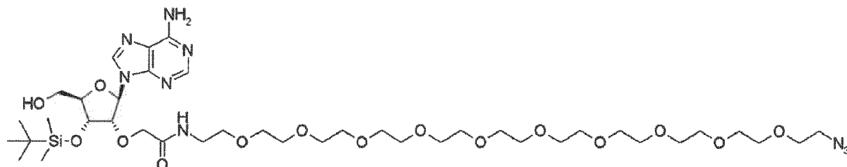
[Compound 11]
