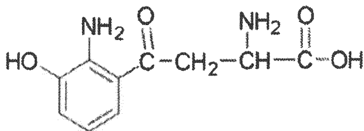
[Compound 3]
