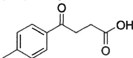
[Compound 21]
