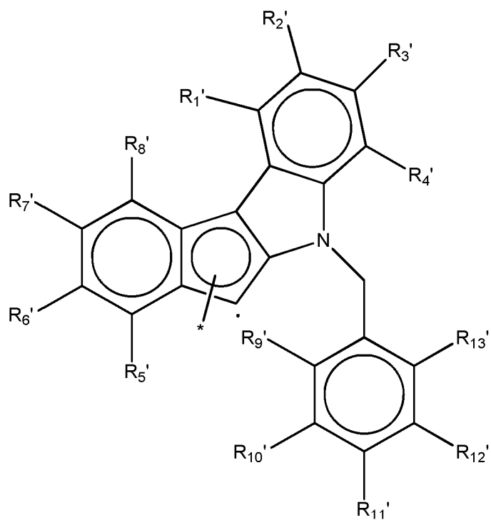
[Chemical Formula 2c]
