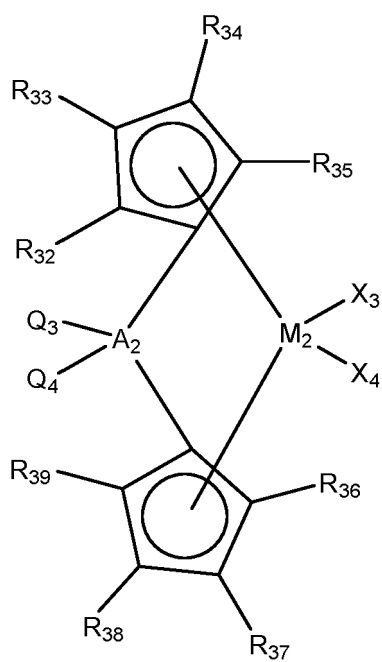
[Chemical Formula 3-2]
