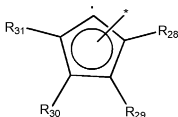
[Chemical Formula 2e]
