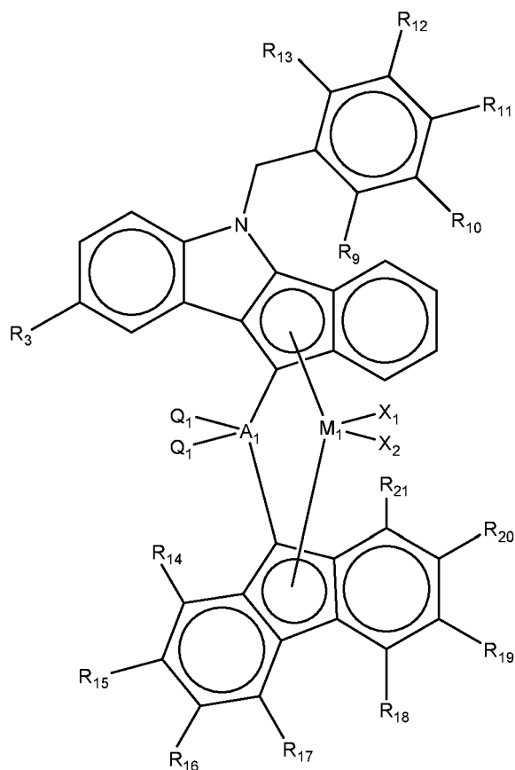
[Chemical Formula 1-1]
