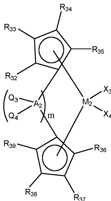
[Chemical Formula 3]
