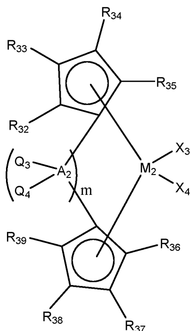
[Chemical Formula 3]
