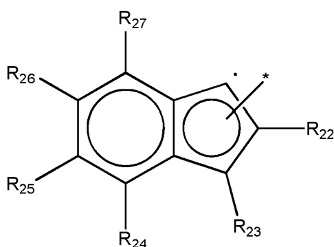
[Chemical Formula 2e]
