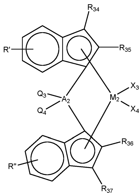
[Chemical Formula 3-4]
