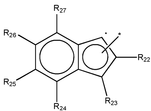
[Chemical Formula 2d]
