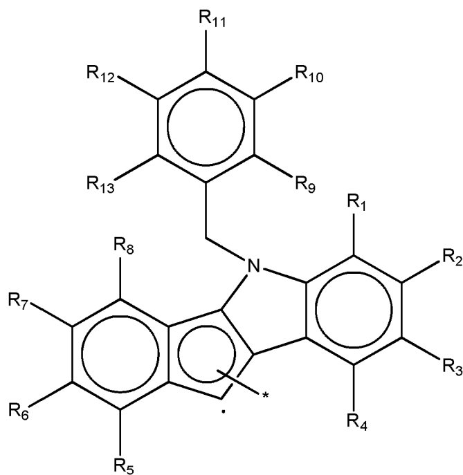
[Chemical Formula 2a]
