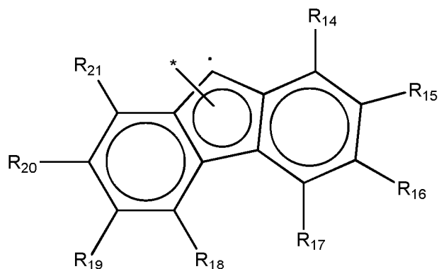
[Chemical Formula 2d]
