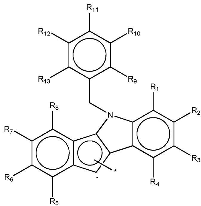
[Chemical Formula 2b]
