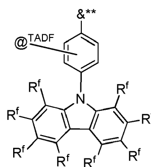
Formula B3*
