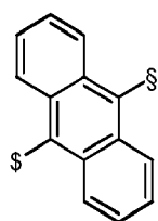
Formula L29
