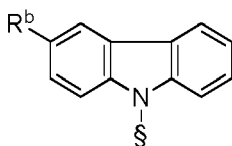
Formula IIcq
