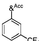
Formula A11
