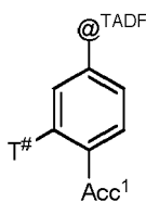
Formula LmT
