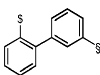
Formula L11
