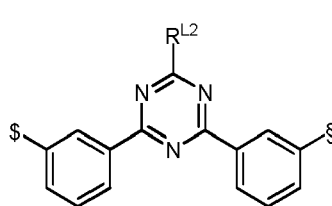
Formula L14
