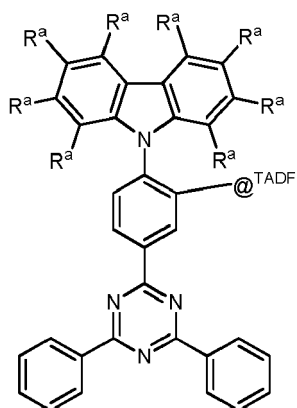
Formula M^{TADF} -1
