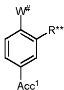
Formula WoL
