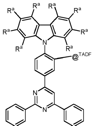
Formula M^{TADF} -3
