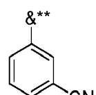
Formula A8**
