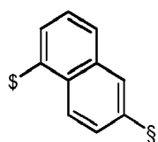
Formula L33
