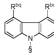
Formula IIbq-4
