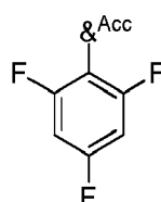
Formula A22
