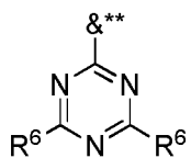
Formula A1**
