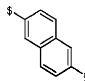
Formula L34
