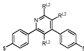
Formula L26
