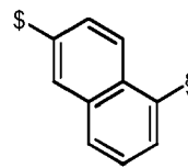
Formula L34
