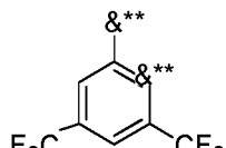
Formula A16**
