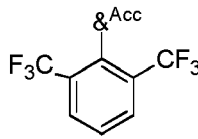
Formula A18
