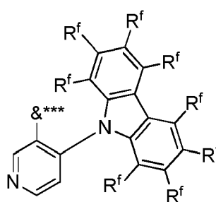
Formula B8**
