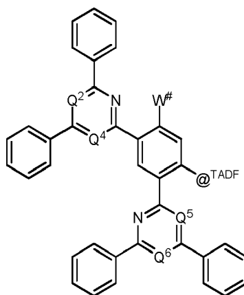
Formula lab
