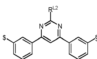
Formula L17
