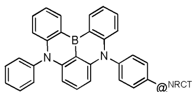
Formula M^{NRCT} -4
