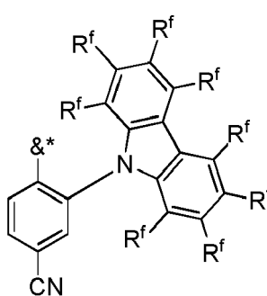
Formula B5
