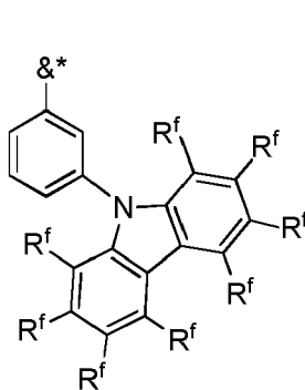
Formula B2
