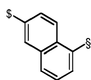
Formula L34
