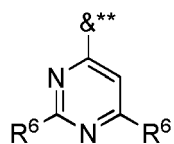
Formula A2**
