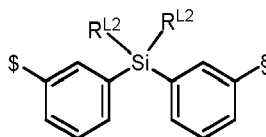
Formula L36
