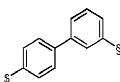
Formula L5
