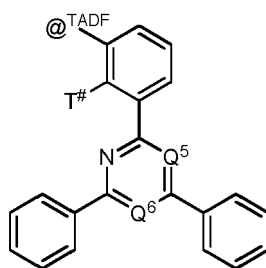
Formula LoT-I
