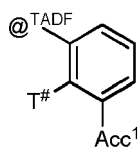
Formula LoT
