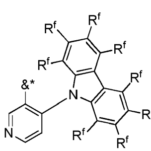
Formula B8
