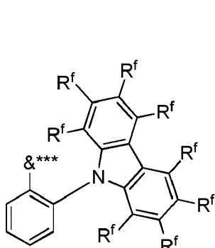
Formula B1**
