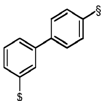
Formula L7
