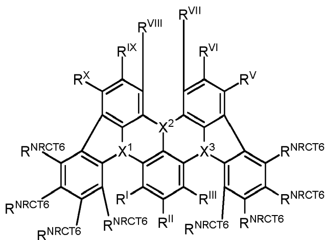
Formula NRCT-Cbz
