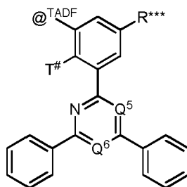
Formula LTP-I
