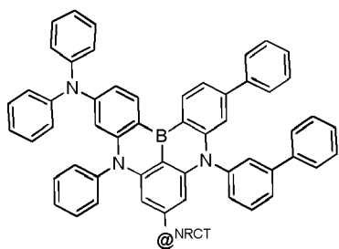
Formula M^{NRCT} -7
