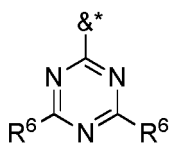
Formula A1*
