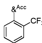
Formula A10
