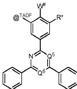
Formula LWo-I
