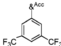
Formula A16
