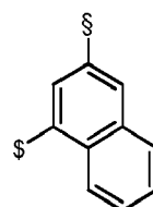
Formula L31
