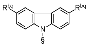
Formula IIbq
