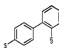
Formula L6
