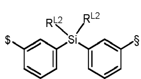
Formula L36
