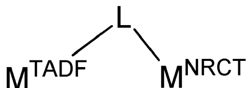
Formula A
