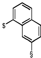
Formula L33
