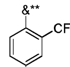
Formula A17**
