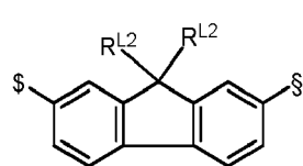
Formula L39
