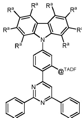
Formula M^{TADF} -4
