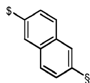
Formula L34
