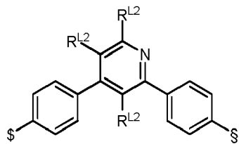
Formula L27
