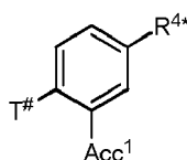
Formula TpL
