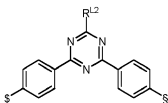
Formula L13
