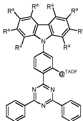
Formula M^{TADF} -2
