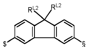
Formula L38
