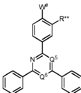
Formula WoL-I
