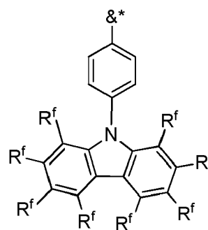
Formula B3
