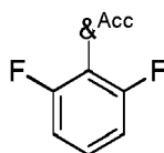
Formula A21
