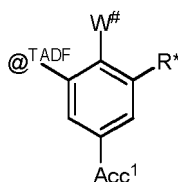
Formula LWo
