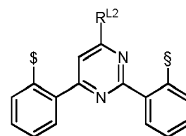
Formula L24
