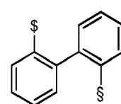
Formula L12
