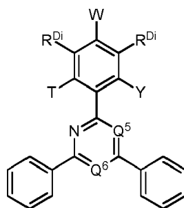
Formula Ia
