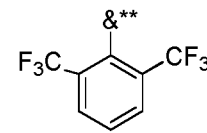
Formula A18**
