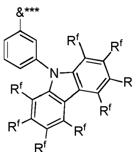
Formula B2**
