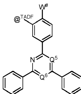
Formula WoT-I
