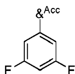
Formula A19
