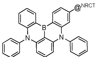
Formula M^{NRCT} -5
