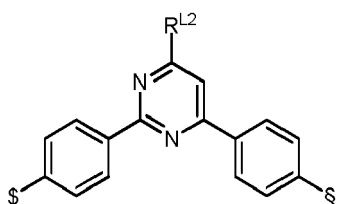
Formula L19
