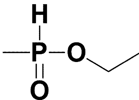
<Chemical Formula 13>
