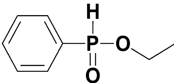
<Chemical Formula 14>
