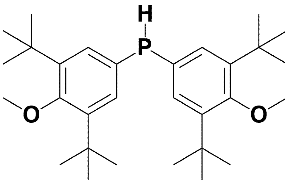
<Chemical Formula 8>
