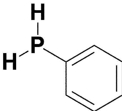
<Chemical Formula 5>
