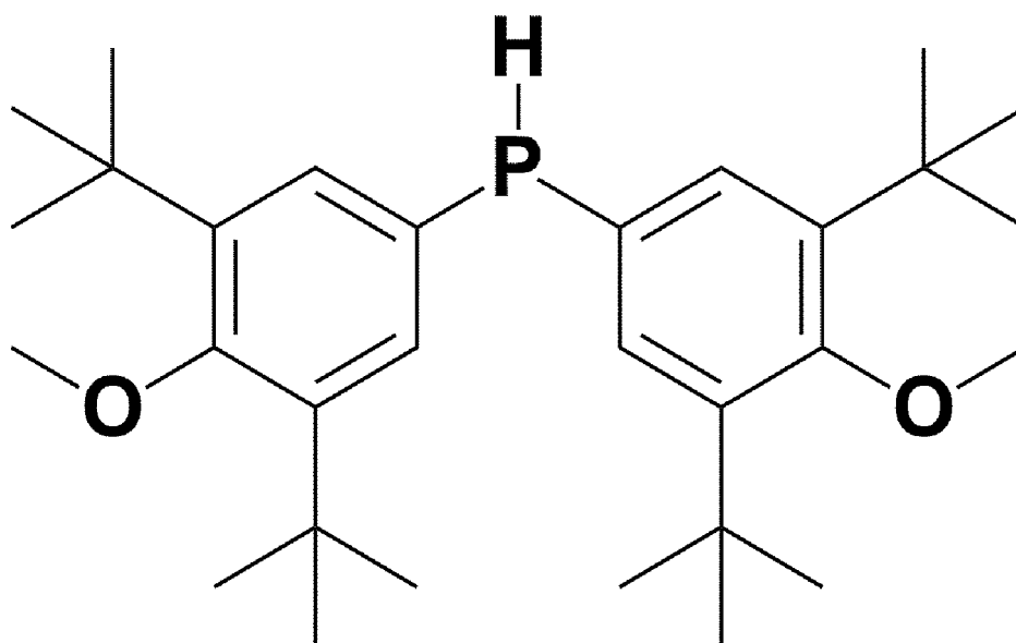
<Chemical Formula 7>
