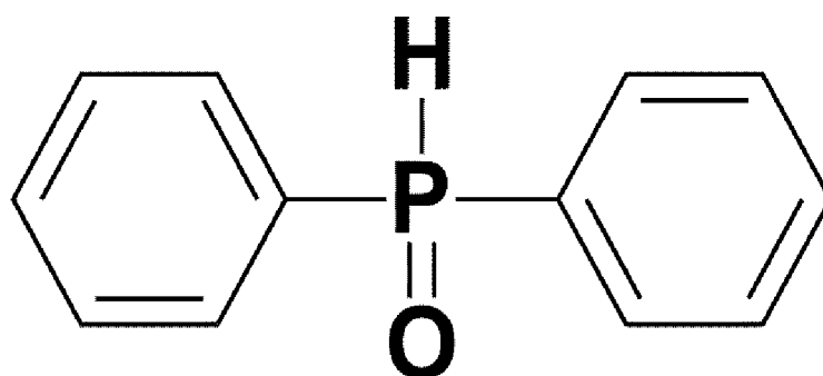
<Chemical Formula 8>
