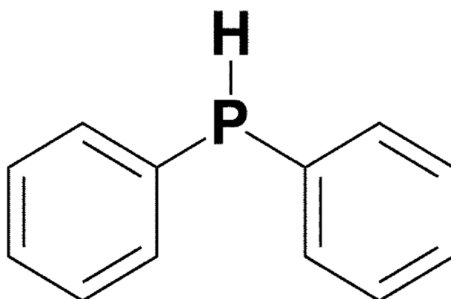
<Chemical Formula 6>
