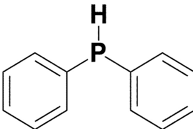
<Chemical Formula 7>
