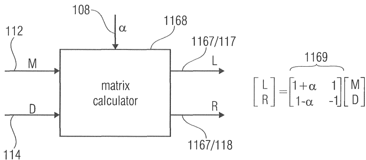
FIG 4B (AUDIO DECODER SIDE)
