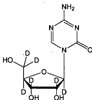
I-7
