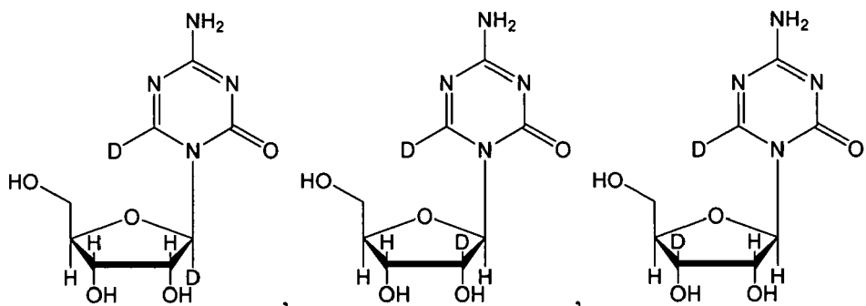
I-9
