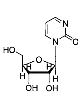
Zebularine
