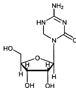
5-6-Dihydro-5-azacytidine
