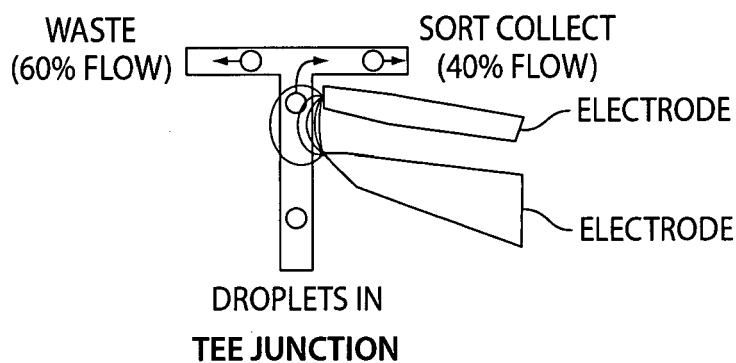
TEE JUNCTION
