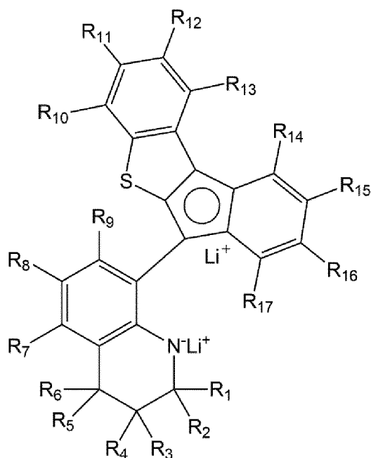
[Formula 6]
