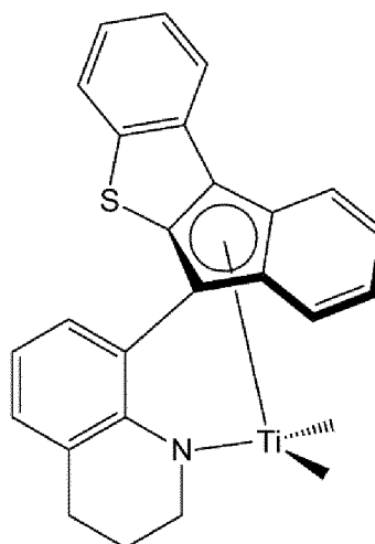
[Formula 1-2]
