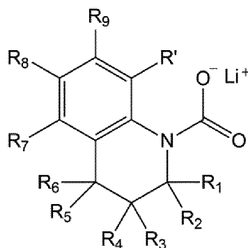
[Formula 3a]
