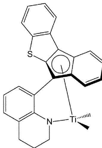
[Formula 1-2]
