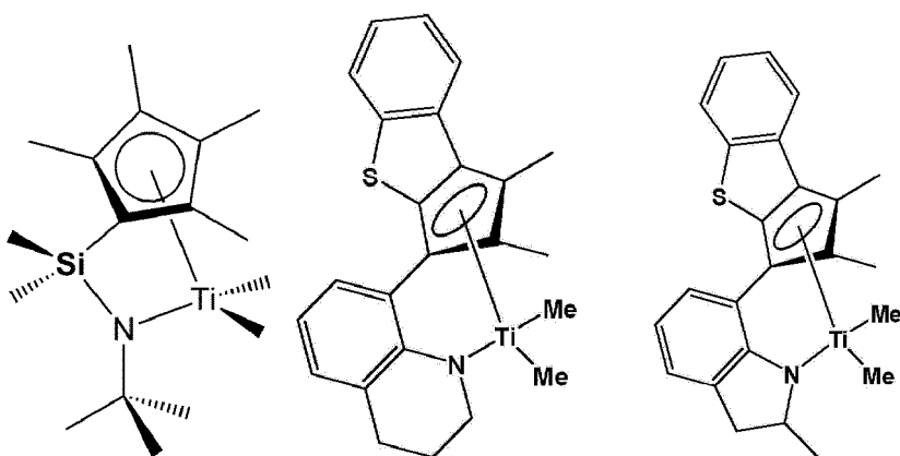
[Compound D]
