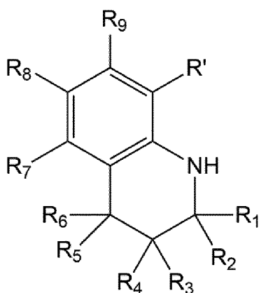
[Formula 2]
