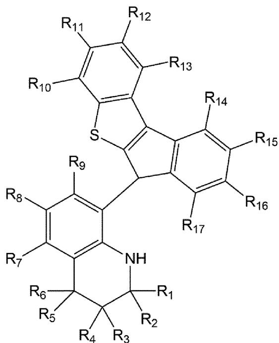
[Formula 6]
