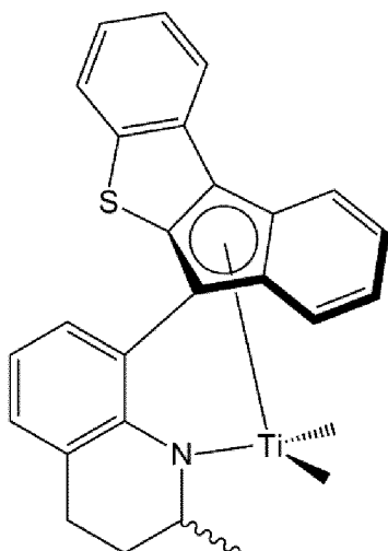
[Formula 1-1]
