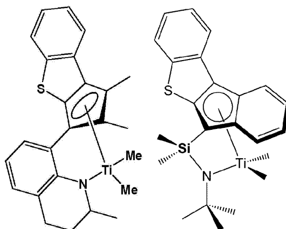
[Compound D]
