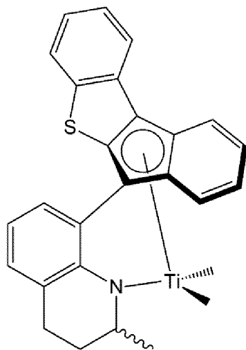
[Formula 1-1]
