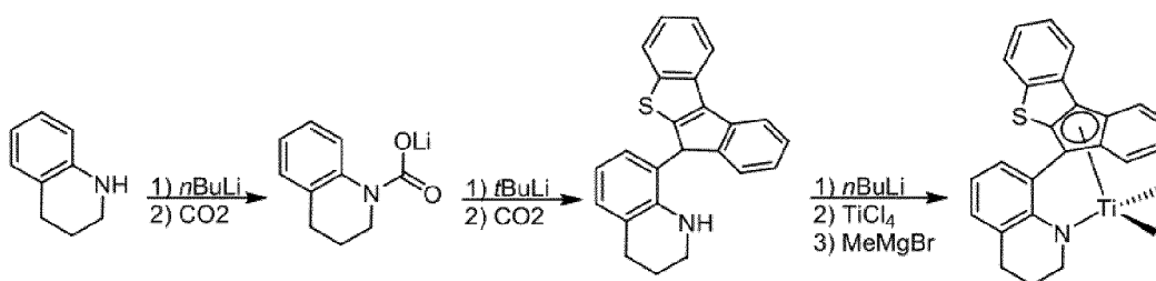
[Reaction 1]
