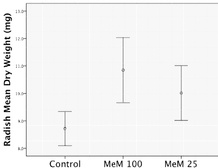
FIG. 8. Immersion of radish sprouts in MeM resulted in significantly increased whole plant mean dry weights of approximately 17% and 11% over the population of the Nutrient Control in 48 h. Error bars indicate \pm SE Control 0.3; MeM 100 0.6; MeM 25 0.5.
