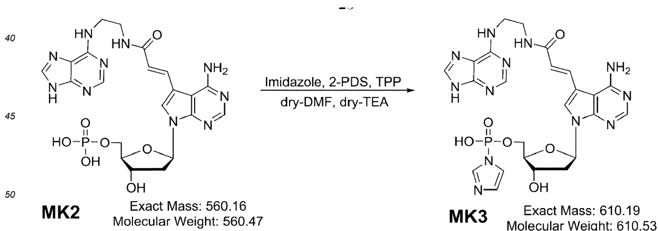
Scheme 3
