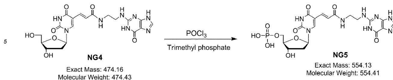
Scheme 10
