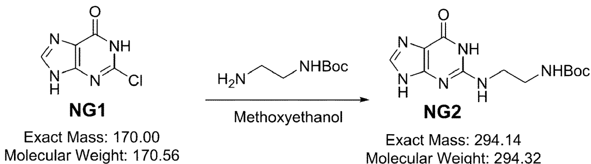
Scheme 7
