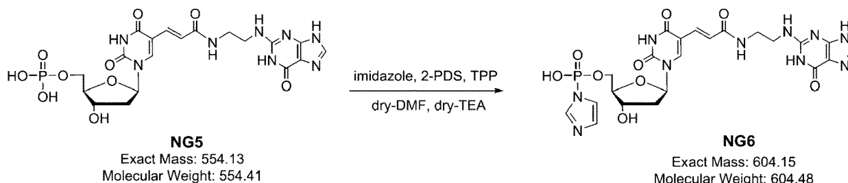
Scheme 11
