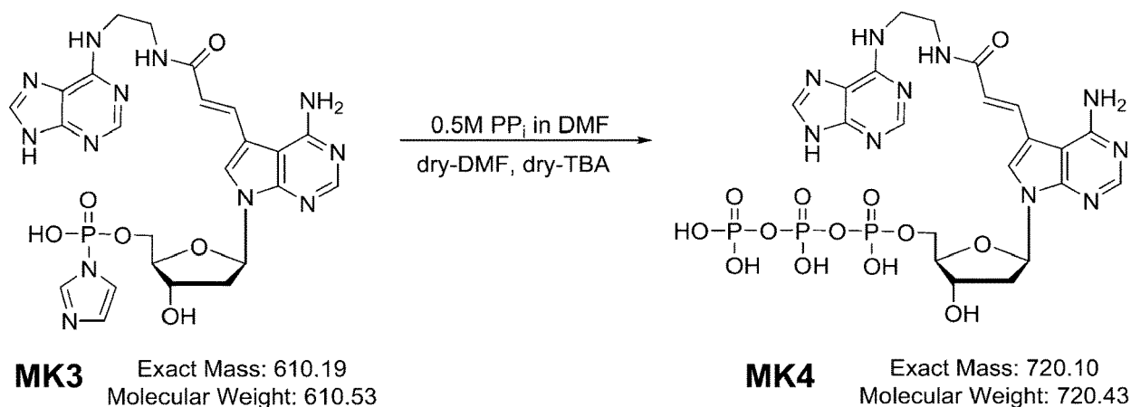
Scheme 4
