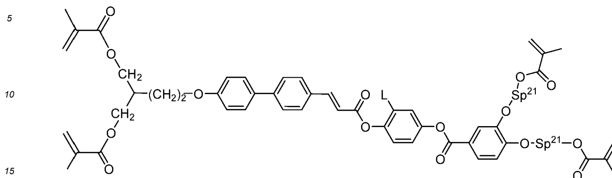
I-4-1a-8-1
