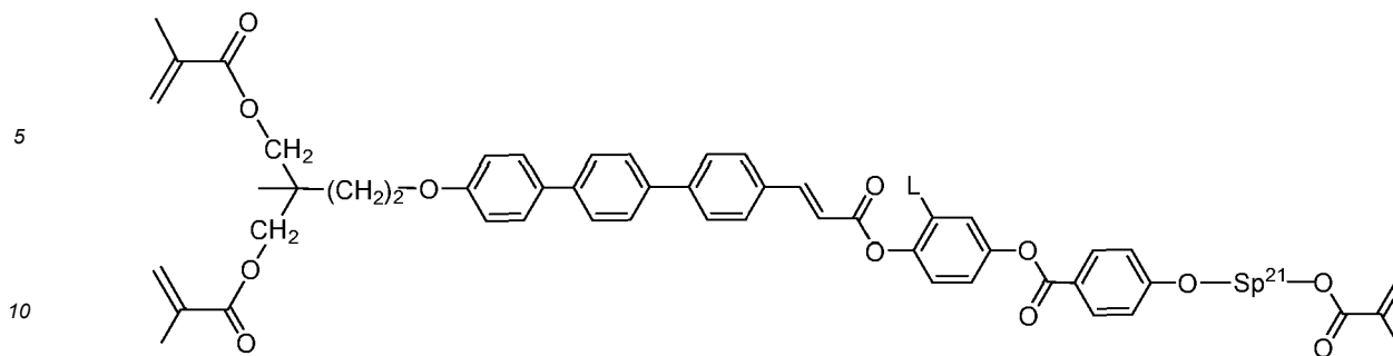
I-5-1a-21
