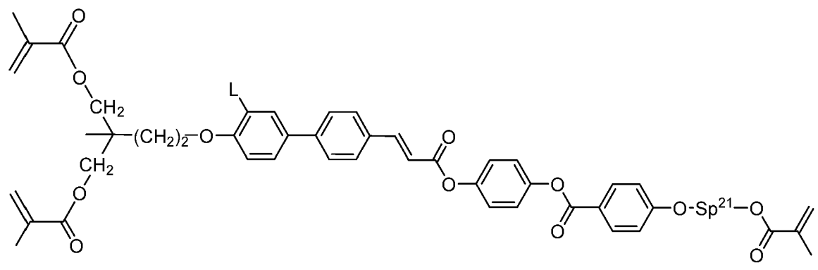
I-4-1a-13
