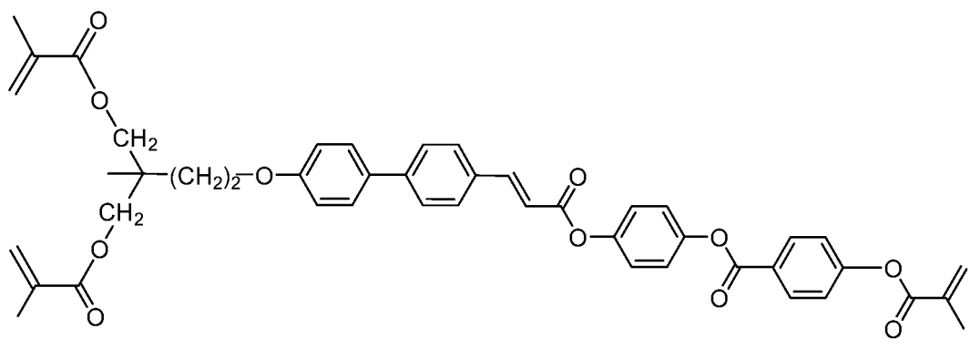
I-4-1a-12
