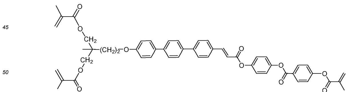
I-5-1a-16
