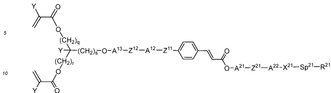
I-5-1
