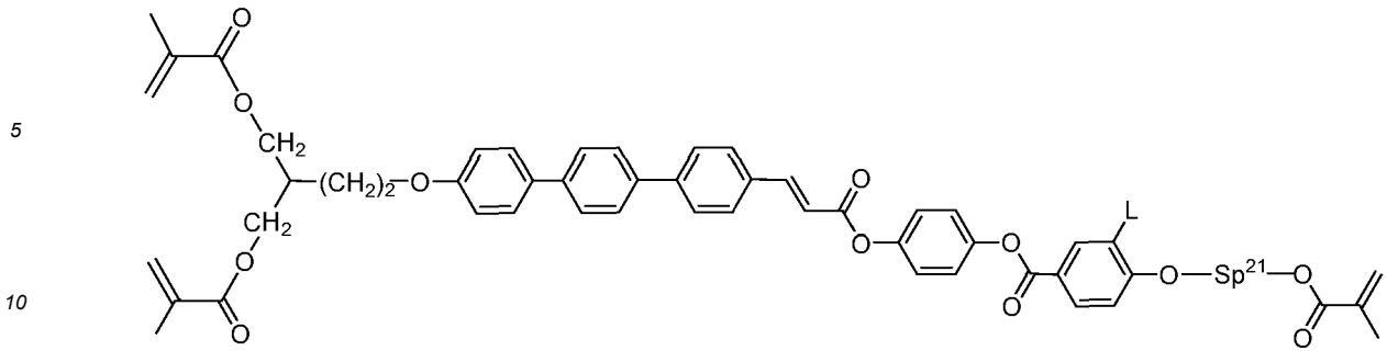
I-5-1a-13
