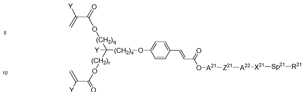
I-3-1
