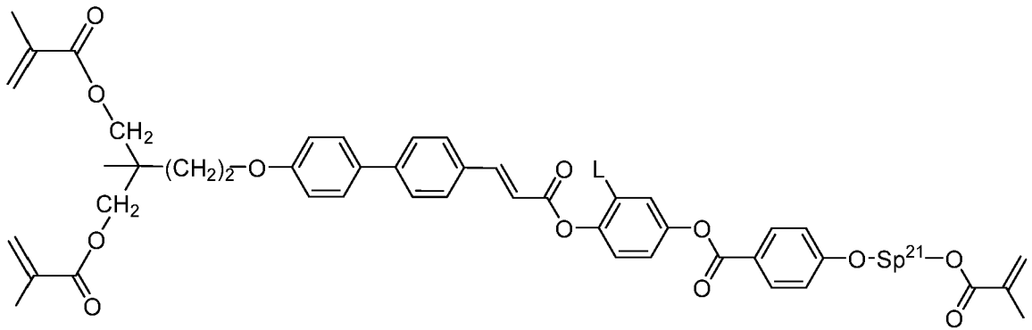
I-4-1a-17
