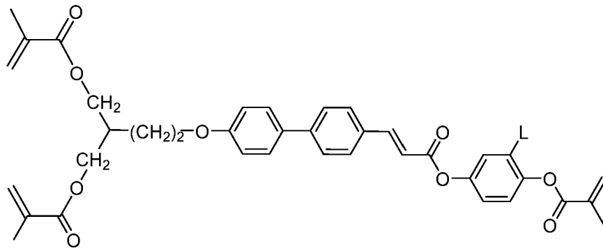
I-2-1a-8
