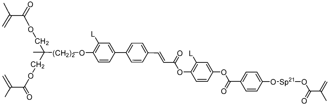
I-4-1a-15
