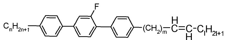
PGP-n-mVI
