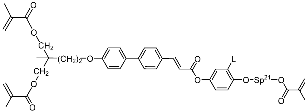
I-2-1a-14
