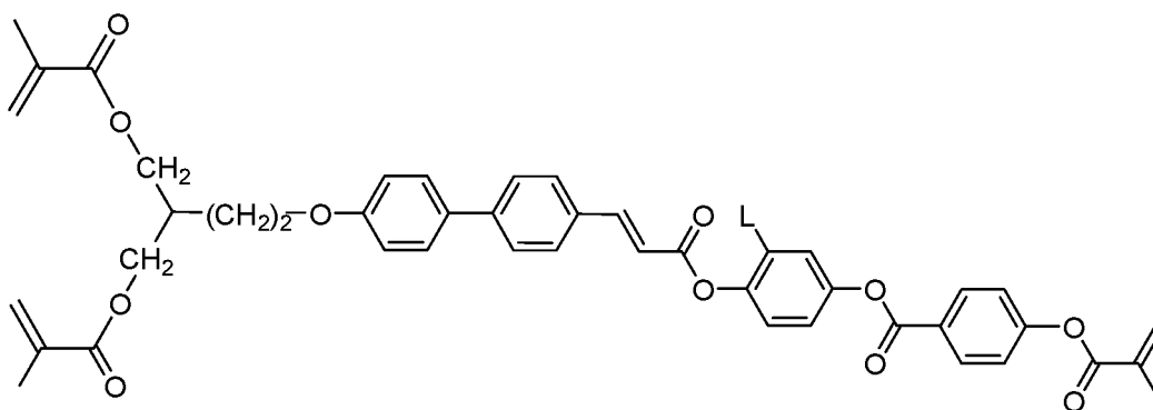
I-4-1a-8
