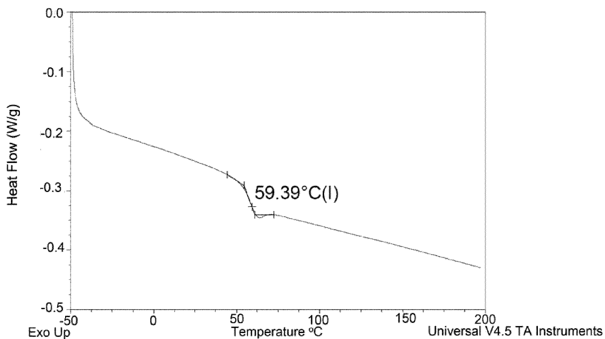
FIG. 2 DSC curve of homopolymer 2-phenyl-1-propyl ethyl methylene malonate.
