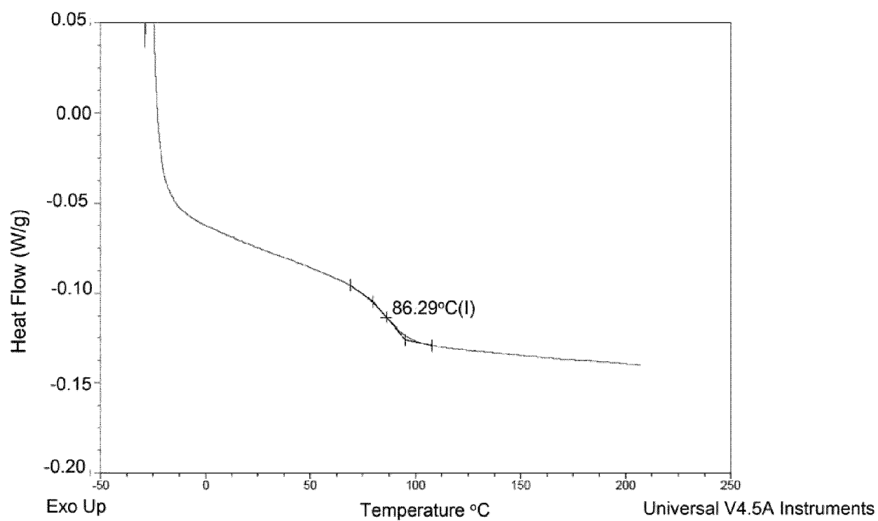
FIG. 4. DSC Curve of homopolymer random copolymer of 2-phenyl-1-propyl ethyl methylene malonate (about 50 weight percent) and fenchyl methyl methylene malonate (about 50 weight percent).
