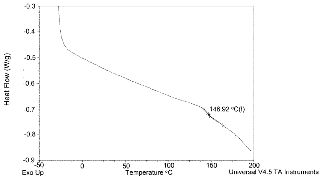
FIG. 3. DSC curve of homopolymer of fenchyl methyl methylene malonate.
