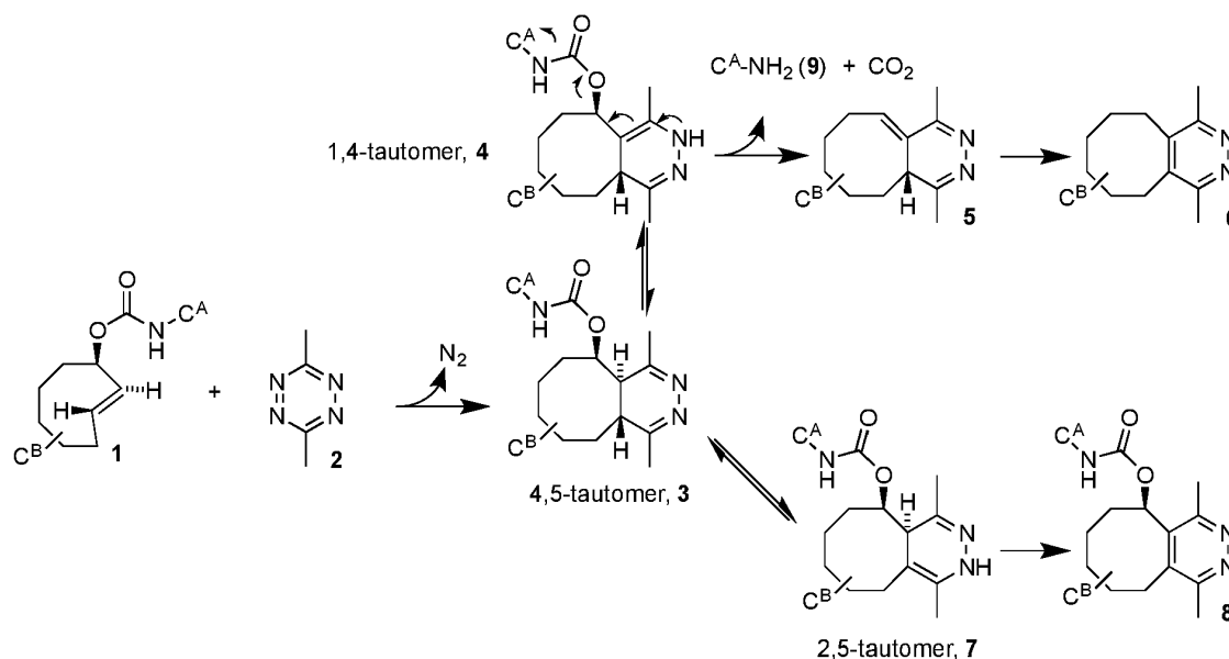
Scheme 2. Proposed IEDDA pyridazine elimination mechanism.
