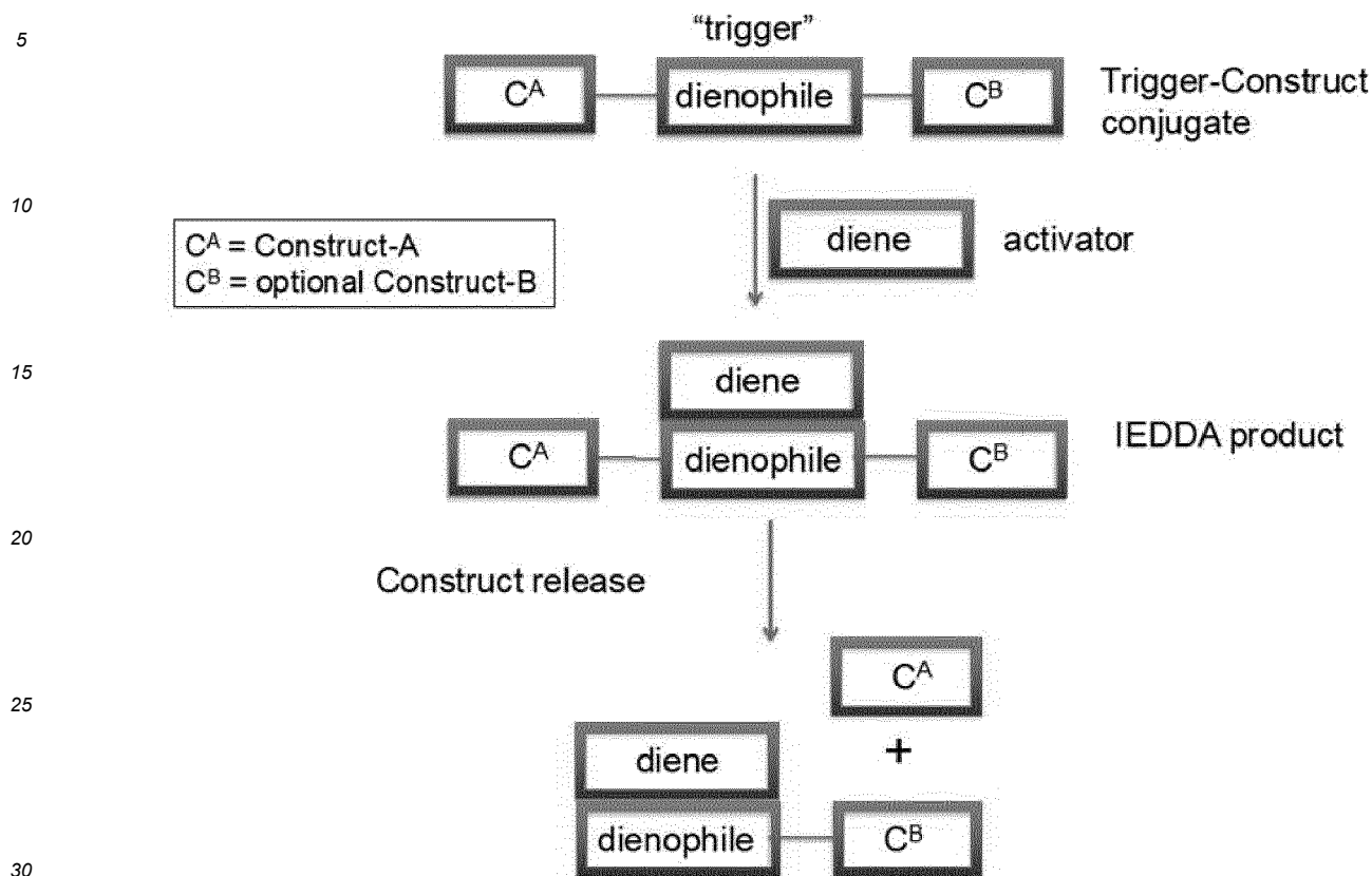
Scheme 3: General scheme of IEDDA pyridazine elimination reaction for the release of Construct-A according to this invention
