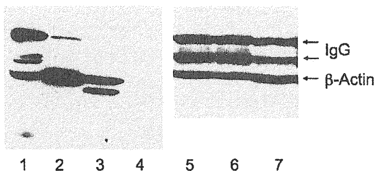
Figure 13. Protein stabilisation.
