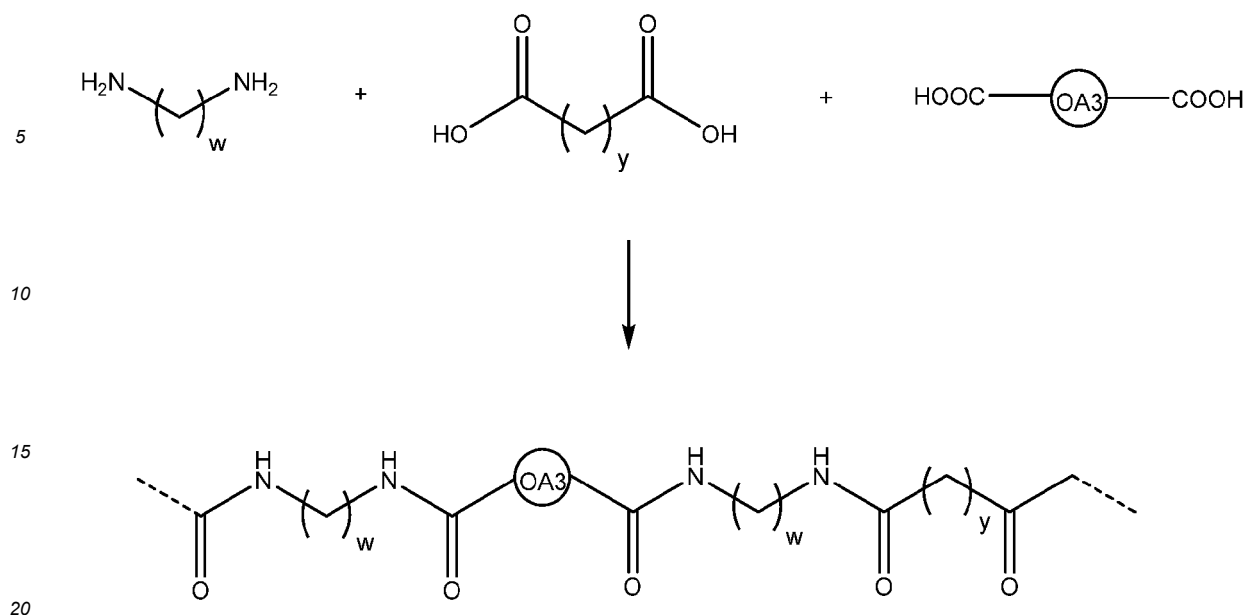
Scheme 7
