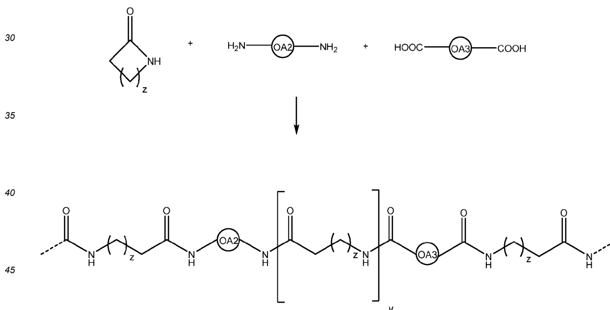
Scheme 11
