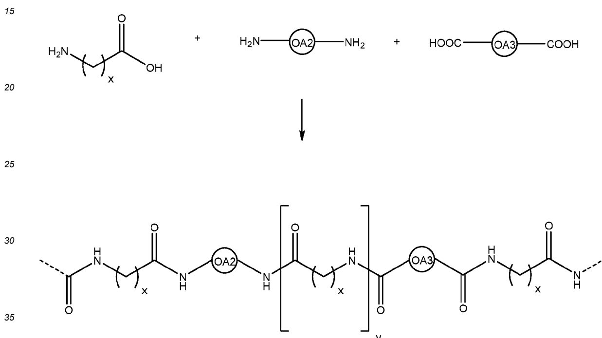
Scheme 4
