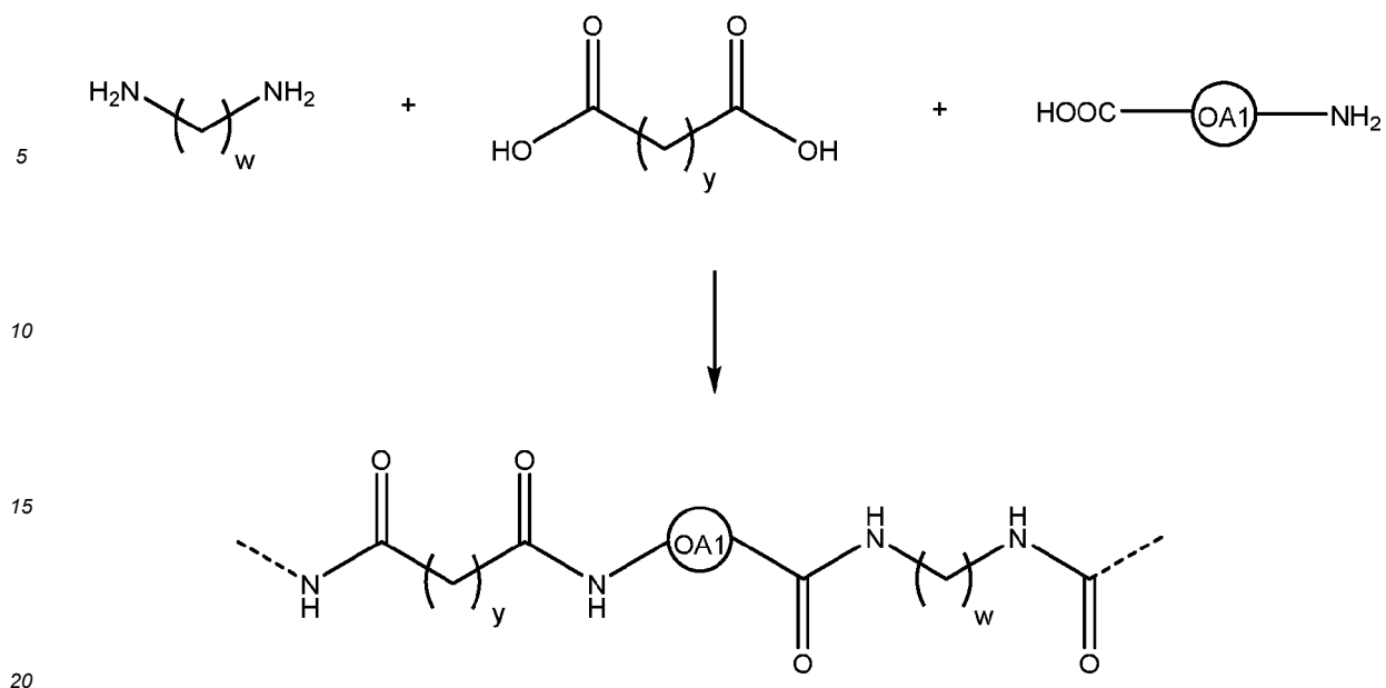
Scheme 5
