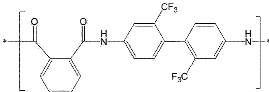
[Chemical Formula 2-5]
