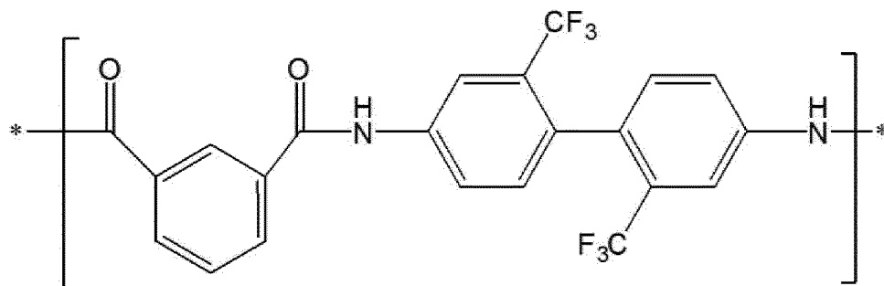
[Chemical Formula 2-4]
