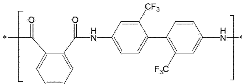
[Chemical Formula 2-5]
