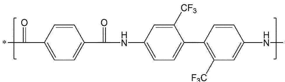
[Chemical Formula 1-1]
