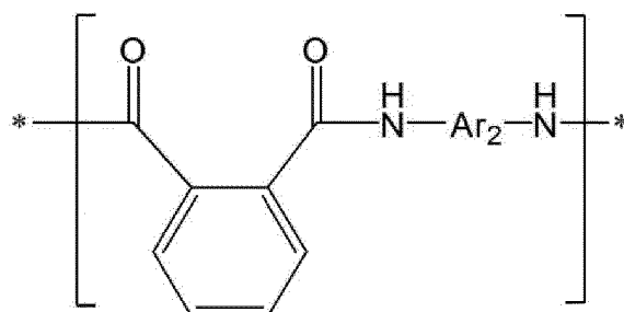
[Chemical Formula 2-2]
