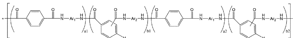
[Chemical Formula 4]
