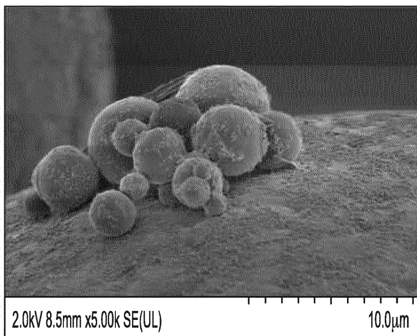
FIG. 13D
