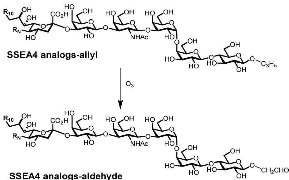
Scheme 6.
