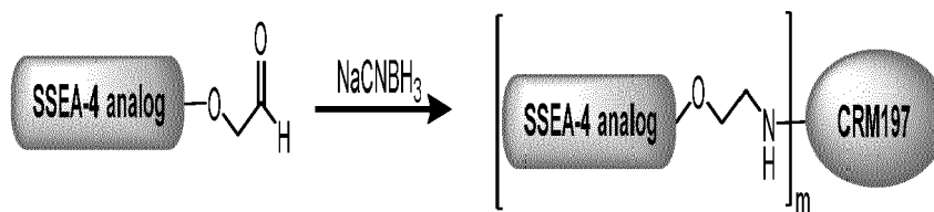
Scheme 10
