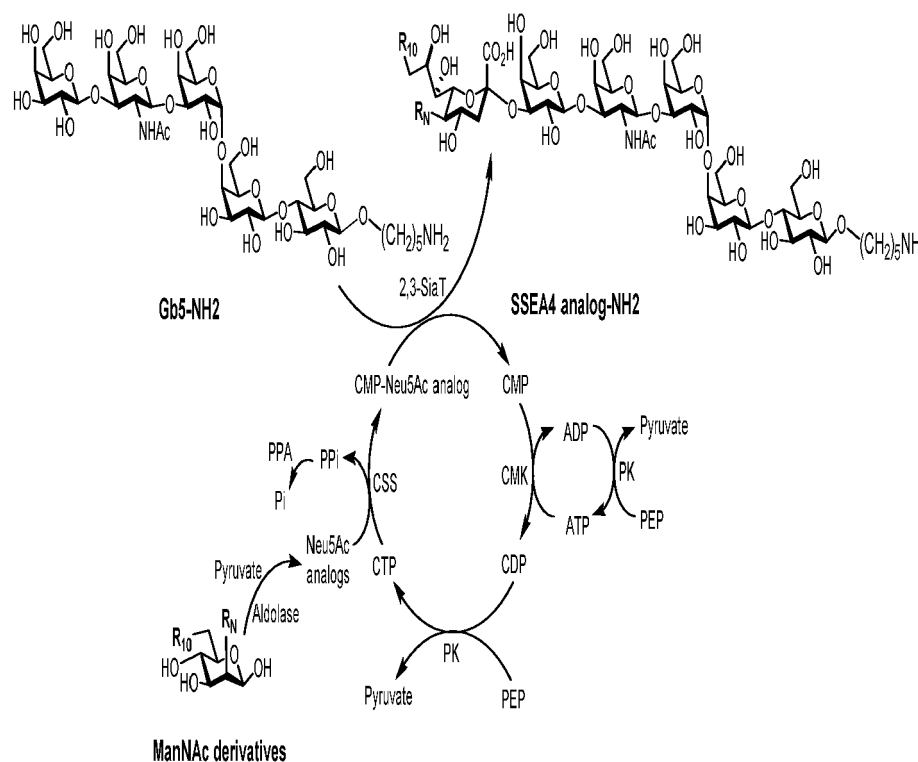
Scheme 3. Synthesis pathway of SSEA4 analog-NH 2 by regeneration system
