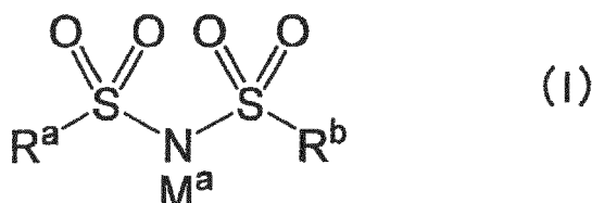
[Chemical Formula 1]
